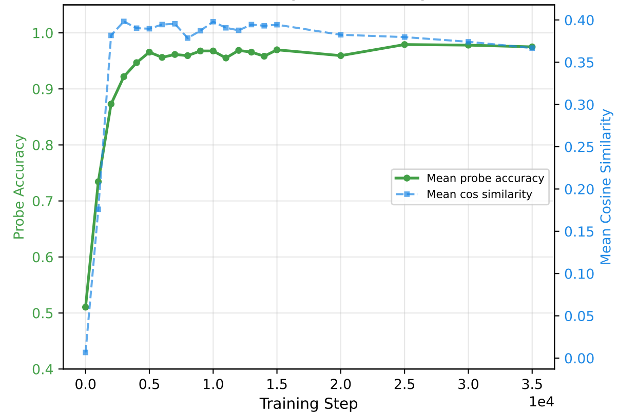
(c) Accuracy vs. Geometry
