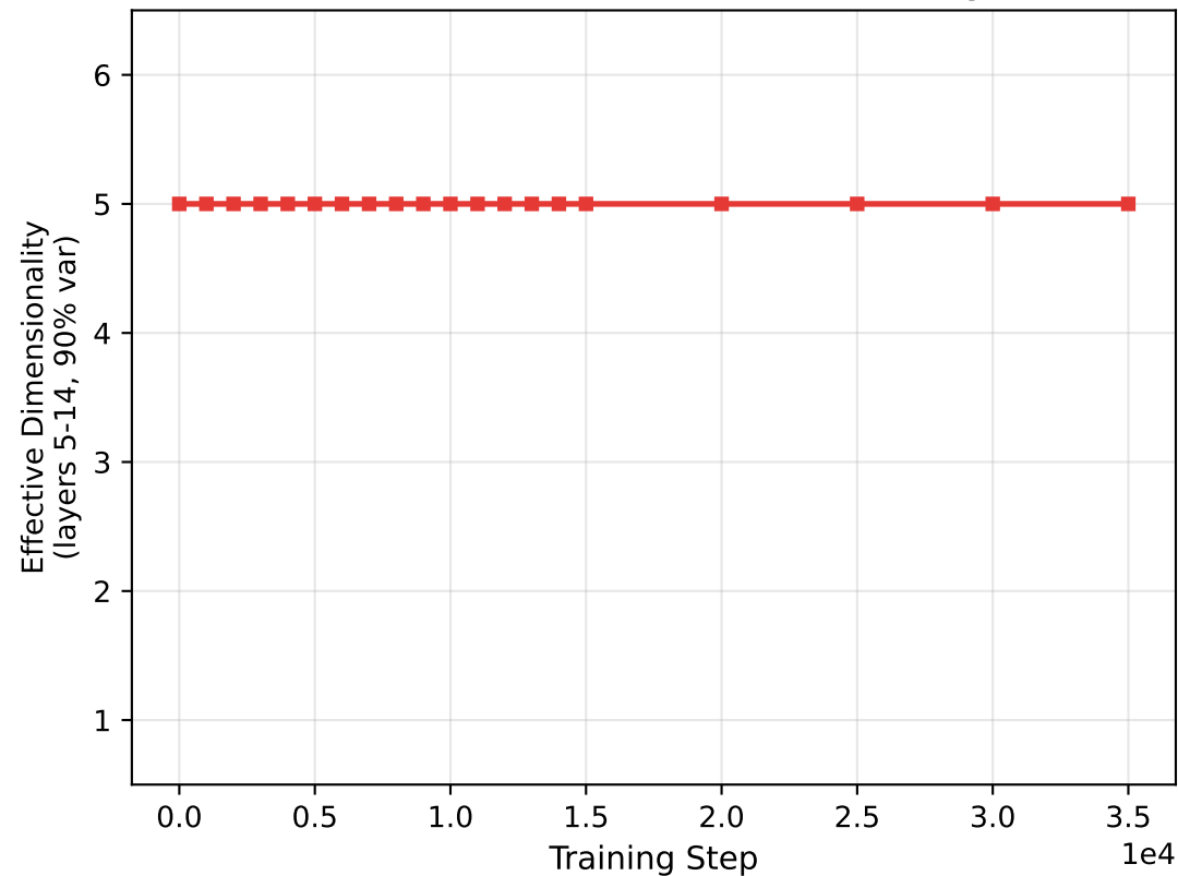
(b) Framework Direction Diversity
