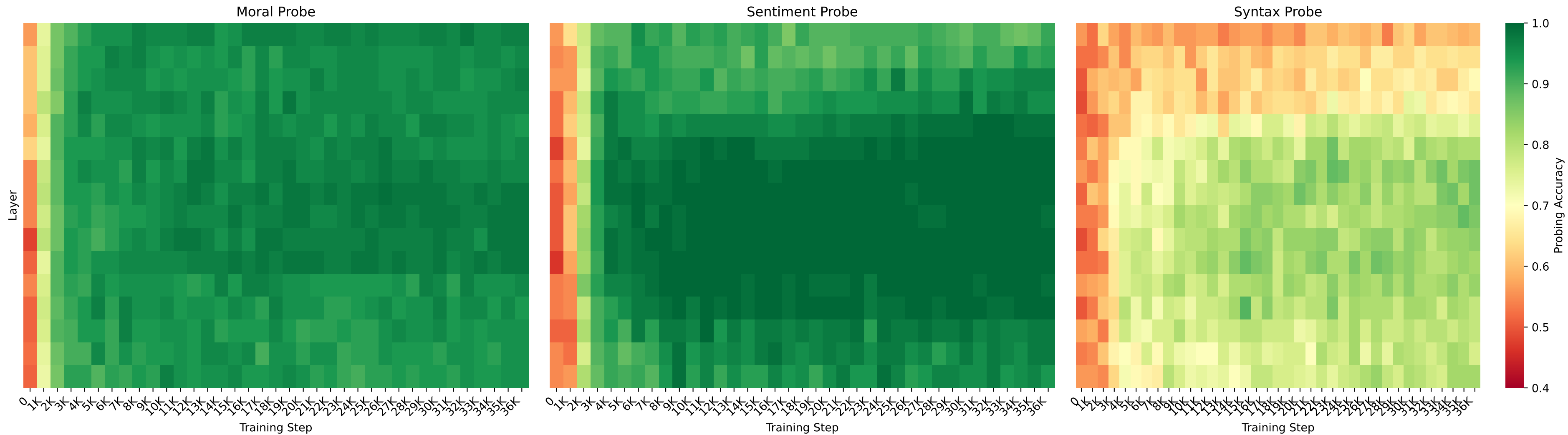
Figure 8b: Per-Layer Emergence Patterns — allenai/OLMo-2-0425-1B-early-training
