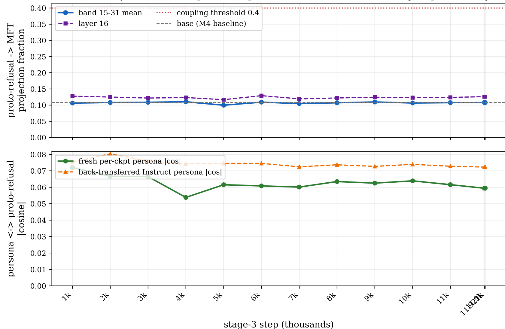
Malleability: how MFT-shaped is the proto-refusal contrast across stage-3 pre-training
