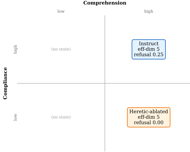
Figure 5: The dissociation matrix, populated. The low-comprehension column is empty: every OLMo-3 state has full comprehension (effective dimensionality 5). The two populated cells differ only in compliance (refusal rate on harmful requests): Instruct refuses, the refusal-ablated model does not.
