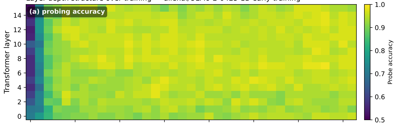
Layer-depth structure over training --- allenai/OLMo-2-0425-1B-early-training
