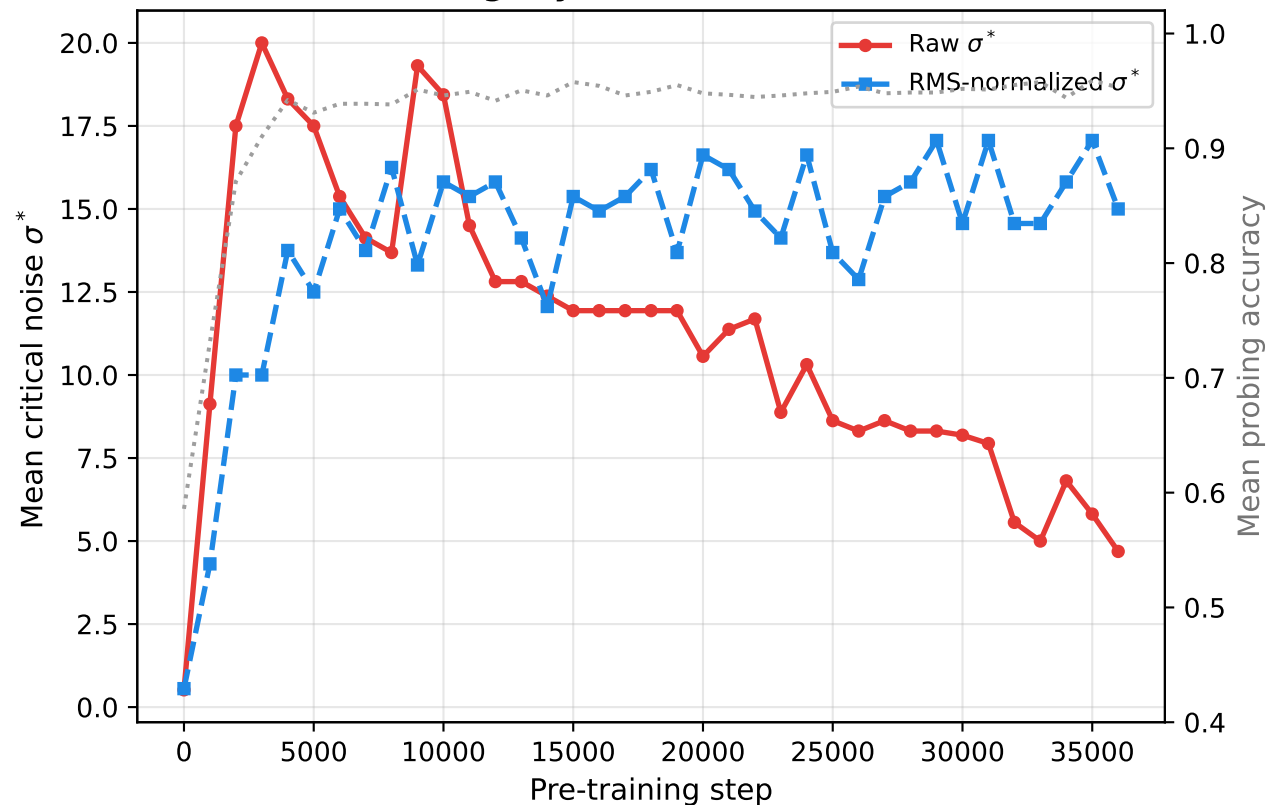
(a) Mean fragility: raw declines, RMS is flat
