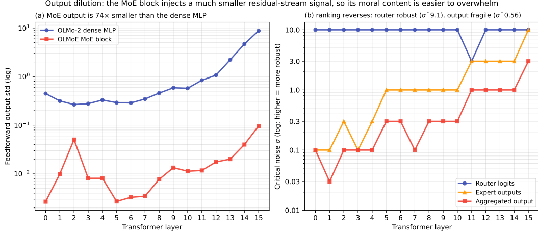
Figure 3: Output dilution explains MoE fragility. (a) Per-layer feedforward output scale (standard deviation of the mean-pooled output) for the OLMoE MoE block vs. the dense OLMo-2 MLP; the dense MLP output is 74\times larger on average. (b) Per-layer critical noise for the three MoE perturbation targets: the router is most robust (mean \sigma^* 9.1 ), the aggregated output most fragile (mean \sigma^* 0.56 ), because the output operates on the diluted scale from panel (a).
