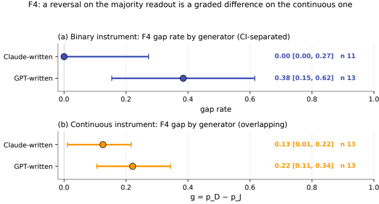
Figure 5: F4 by generator. (a) On the majority readout the Claude-written and GPT-written halves of F4 are CI-separated (0.00 vs 0.38); (b) on the continuous readout they overlap (0.13 vs 0.22). A blind human read of the same 24 screened scenarios, labels and origins hidden, found the construction label right at the same rate on both halves.
