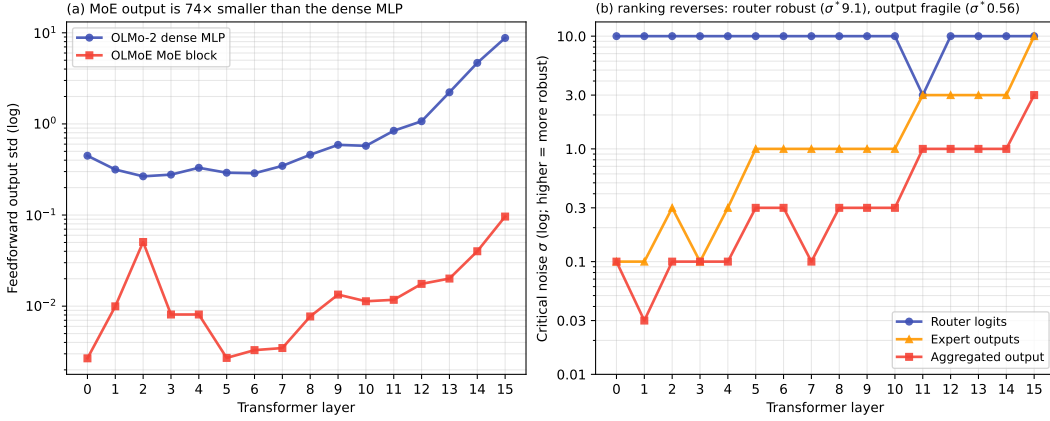
Figure 3: Output dilution explains MoE fragility. (a) Per-layer feedforward output scale (standard deviation of the mean-pooled output) for the OLMoE MoE block vs. the dense OLMo-2 MLP; the dense MLP output is 74\times larger on average. (b) Per-layer critical noise for the three MoE perturbation targets: the router is most robust (mean \sigma^* 9.1 ), the aggregated output most fragile (mean \sigma^* 0.56 ), because the output operates on the diluted scale from panel (a).
