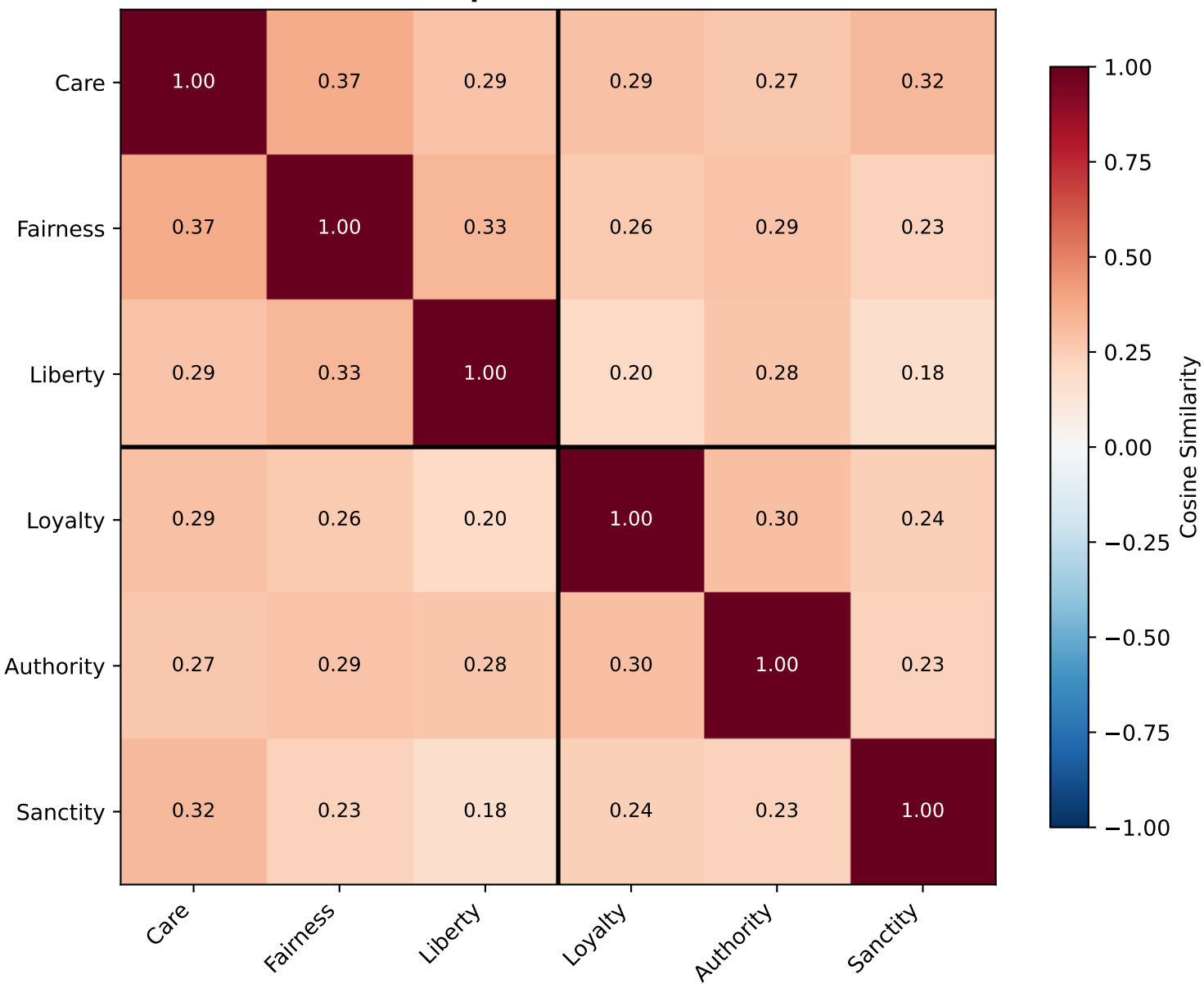
Foundation Probe Direction Cosine Similarity (Layer 0) Mean pairwise = 0.2719
