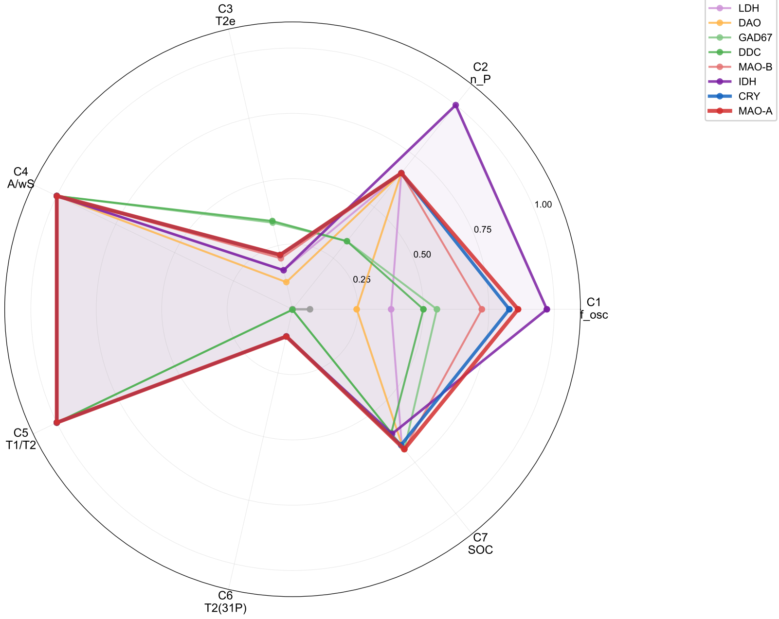
RPM Condition Assessment (7 conditions, normalised scores)
