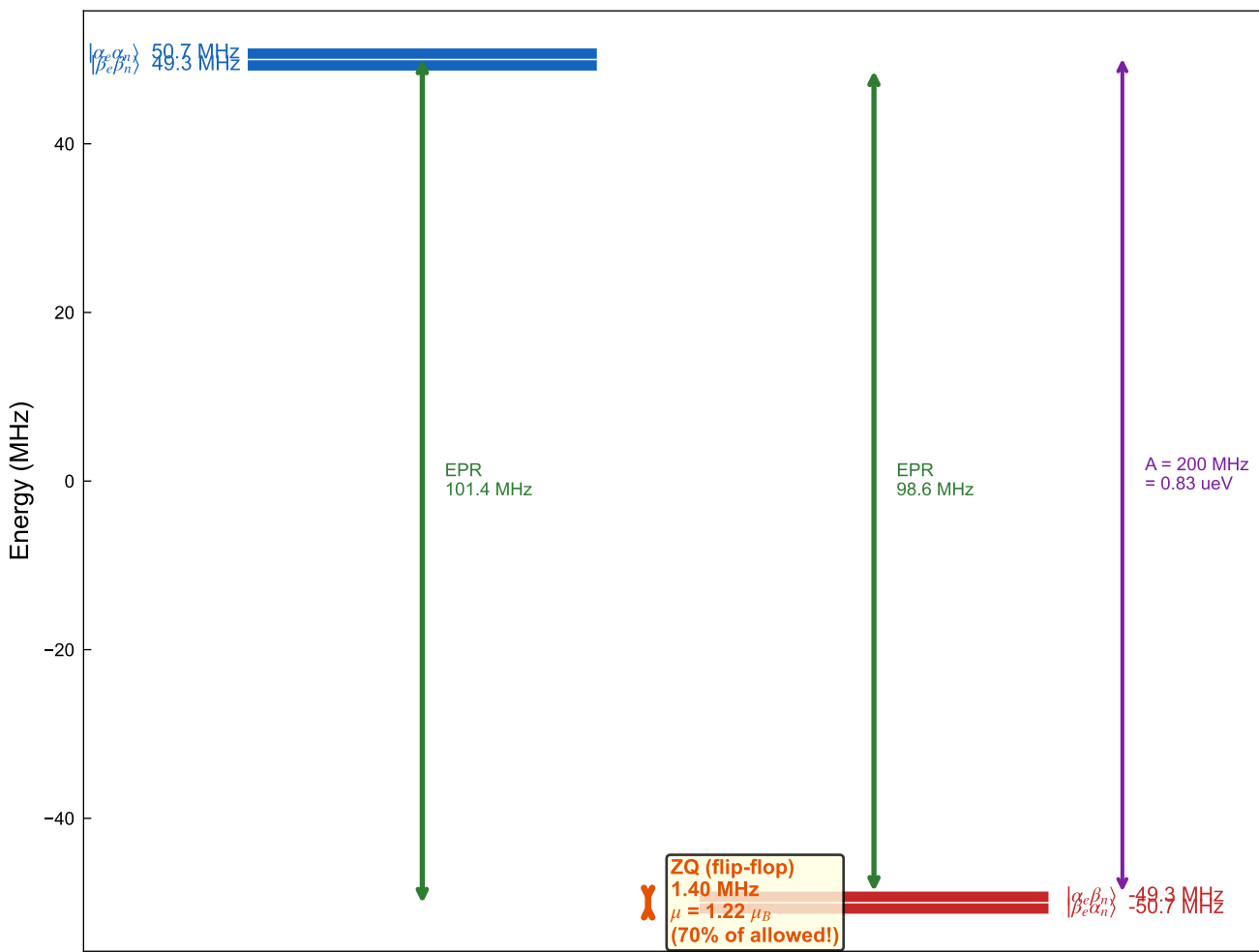
(a) Coupled e^{-}-^{31}\text{P} 4-level system @ 50 \mu\text{T} (strong coupling: A \gg \omega_S )
