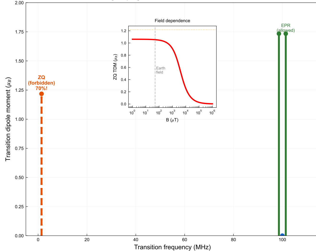
(b) Transition spectrum at 50 \mu\text{T} Strong coupling: forbidden transitions become allowed
