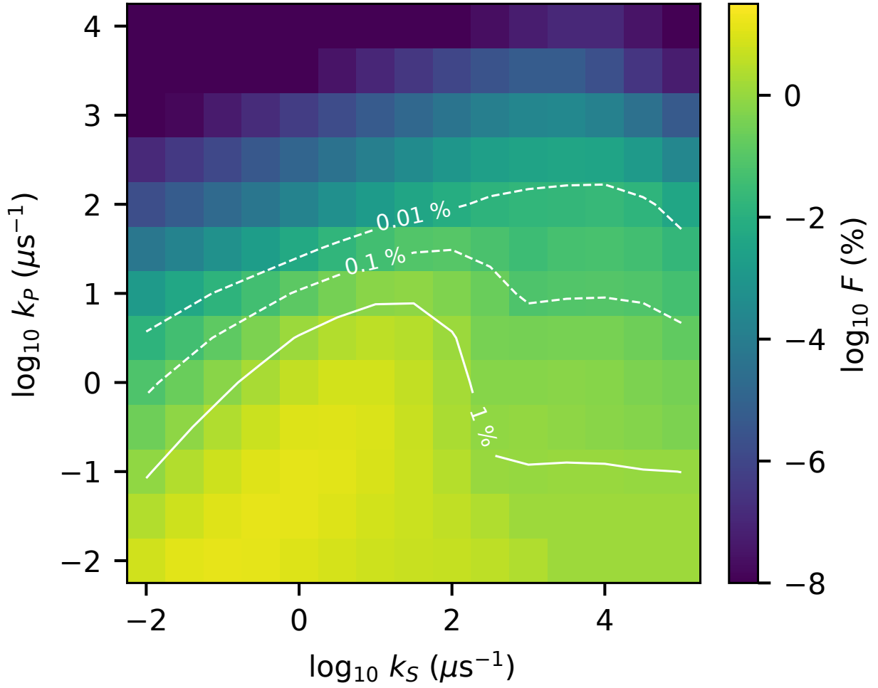
Figure 1: Largest magnetic field effect on the onward yield found by the search over the exchange coupling, the field direction and the dipolar scale s \in [0, 3] , as a function of the singlet back-transfer rate k_S and the spin-independent onward rate k_P . Reference four-nucleus model, coherent spin dynamics, B = 50 \mu\text{T} .
