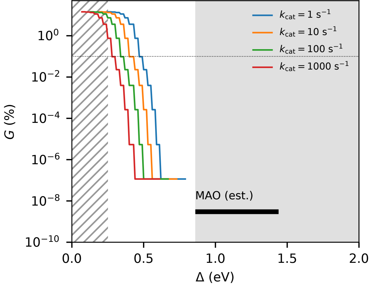
Figure 2: Largest magnetic field effect found by the grid procedure among pairs that can carry the turnover, G(\Delta) , for k_{\text{cat}} = 1, 10, 100 and 10^3 \text{ s}^{-1} in the reference model. Hatched: G not defined for k_{\text{cat}} = 1 \text{ s}^{-1} because the permitted rates extend below the computed grid. Shaded: no pair carries the turnover with \nu_n = 10^{14} \text{ s}^{-1} . Bar: driving force of an amine-to-flavin pair in monoamine oxidase estimated from measured flavin potentials and a proxy amine potential (see the section on monoamine oxidase).
