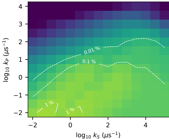
(a) contact dipolar tensor
