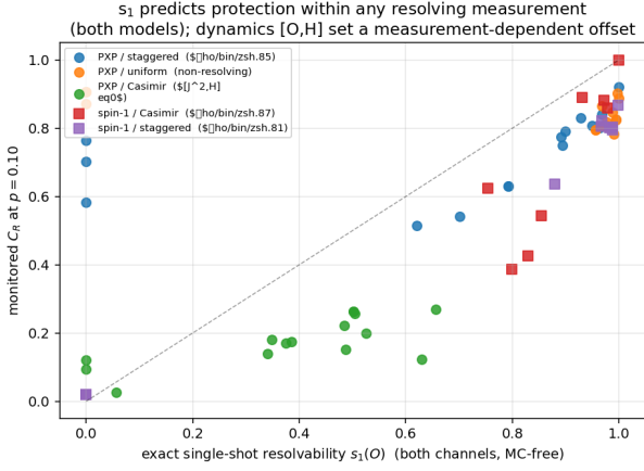
Figure 9: Monitored \mathcal{C}_R ( p = 0.10 ) versus the exact single-shot resolvability s_1(O) for 65 code-measurement pairs across both models. Within each resolving measurement the relation is tight; the non-resolving (uniform) and non-commuting (PXP Casimir) families bound the predictor’s scope.
