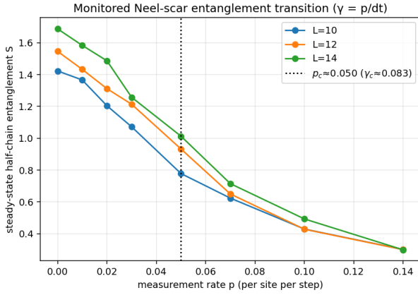
Figure 8: Steady-state half-chain entanglement of the monitored Néel state versus p for L = 10, 12, 14 ; the crossing sets p_c and hence \gamma_c = p_c/dt .
