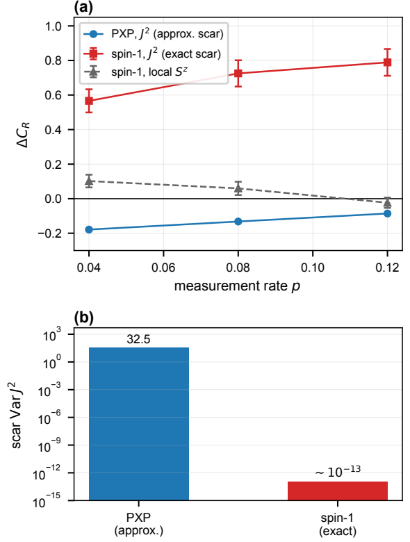
Figure 5: Exact-su(2) scars evade the Casimir-variance obstruction. Second model (spin-1 Schecter-Iadecola, L = 6 , 20-pair thermal ensemble). (a) Scar-thermal coherent information \Delta\mathcal{C}_R versus p (error bars are the ensemble SEM). Under J^2 monitoring PXP scars lose (blue) while exact spin-1 scars win perfectly (red); under generic local S^z the exact-scar and thermal codes are comparable at this size ( |\Delta\mathcal{C}_R| \leq 0.1 , grey; at L = 8 the low-rate difference is larger, +0.20 at p = 0.04 , see text). (b) Scar Casimir variance, \simeq 32 (PXP, canonical rungs; 3.4–47.6 across the tower, always above energy-matched thermal neighbors) versus \sim 10^{-13} (exact) on a log scale—the control parameter of the rescue.
