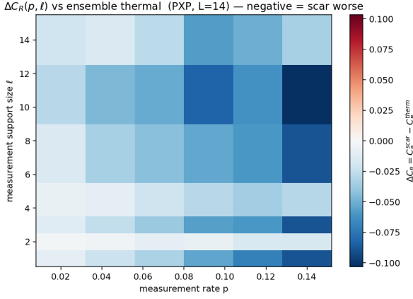
Figure 7: \Delta C_R(p, \ell) against the ensemble thermal baseline (PXP, L = 14 ). Blue is \Delta C_R < 0 (scar worse) everywhere.
