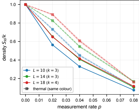
Figure 3: The maximal scar code loses even as an extensive memory. Protected-information density S_R/k for the maximal k = \lfloor \log_2(L+1) \rfloor -qubit scar code (solid) and a same-dimension thermal code (dashed, \pm 1\sigma band) versus p under local monitoring, for L = 10, 14, 18 . Scar lies below thermal throughout.
