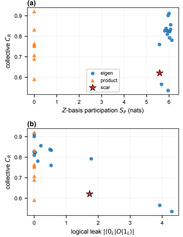
Figure 4: What controls collective protection. Collective \mathcal{C}_R versus (a) Z -basis participation and (b) logical leak |\langle 0_L | O | 1_L \rangle| over an eigenstate sweep (blue), product states (orange), and the canonical scar (star). Higher participation raises \mathcal{C}_R ; large leak suppresses it. The scar is a low- \mathcal{C}_R outlier on both axes.
