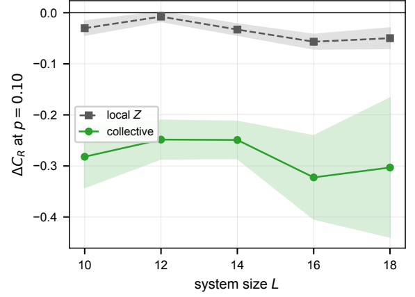
Figure 2: The scar disadvantage \Delta C_R < 0 at every size. Scar-minus-thermal coherent information at p = 0.10 versus L for local (grey) and collective (green) monitoring; shading is the thermal-ensemble spread (12 pairs, 200 trajectories for L = 10 –16; 6 pairs, 120 trajectories for L = 18 ). At L = 16 the overlap ranking selects the other member of the 2.64/2.74 anticrossing doublet than at L = 10 –14; the sign is partner-robust—the alternative partner gives -0.034 (local) and -0.150 (collective) against -0.066 and -0.306 (scripts/l16_partner_check.py).
