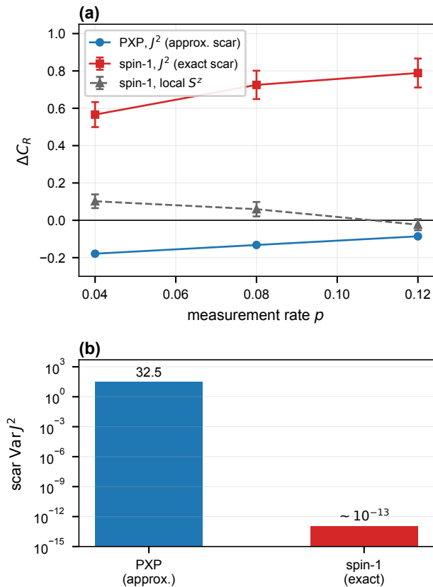
FIG. 5. Exact-su(2) scars evade the Casimir-variance obstruction. Second model (spin-1 Schechter-Iadecola, L = 6 , 20-pair thermal ensemble). (a) Scar–thermal coherent information \Delta C_R versus p (error bars are the ensemble SEM). Under J^2 monitoring PXP scars lose (blue) while exact spin-1 scars win perfectly (red); under generic local S^z the exact-scar and thermal codes are comparable ( |\Delta C_R| \lesssim 0.1 , grey). (b) Scar Casimir variance, \simeq 32 (PXP) versus \sim 10^{-13} (exact) on a log scale—the control parameter of the rescue.
