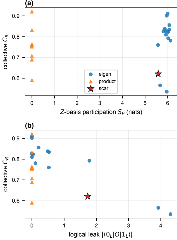
FIG. 4. What controls collective protection. Collective \mathcal{C}_R versus (a) Z -basis participation and (b) logical leak |\langle 0_L | O | 1_L \rangle| over an eigenstate sweep (blue), product states (orange), and the canonical scar (star). Higher participation raises \mathcal{C}_R ; large leak suppresses it. The scar is a low- \mathcal{C}_R outlier on both axes.
