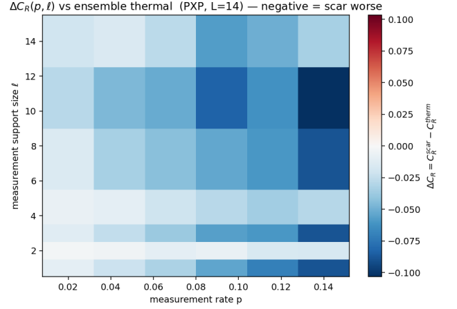
FIG. S2. \Delta\mathcal{C}_R(p, \ell) against the ensemble thermal baseline (PXP, L = 14 ). Blue is \Delta\mathcal{C}_R < 0 (scar worse) everywhere.
