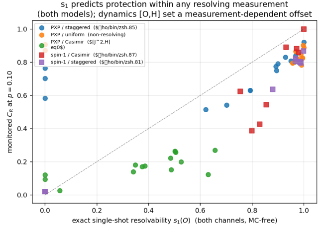
FIG. 10. Monitored \mathcal{C}_R ( p = 0.10 ) versus the exact single-shot resolvability s_1(O) for 65 code–measurement pairs across both models. Within each resolving measurement the relation is tight; the non-resolving (uniform) and non-commuting (PXP Casimir) families bound the predictor’s scope.
