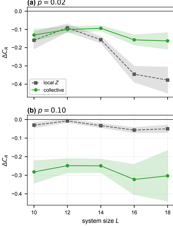
FIG. 2. The scar disadvantage \Delta C_R < 0 at every size. Scar-minus-thermal coherent information versus L for local (grey) and collective (green) monitoring at (a) p = 0.02 , where most information survives and the local deficit grows with size, and (b) the benchmark p = 0.10 ; shading is the thermal-ensemble spread (12 pairs, 200 trajectories for L = 10 –16; 6 pairs, 120 trajectories for L = 18 ). At L = 16 the overlap ranking selects the other member of the 2.64/2.74 anticrossing doublet than at L = 10 –14; the sign is partner-robust—the alternative partner gives -0.034 (local) and -0.150 (collective) against -0.066 and -0.306 at p = 0.10 ( scripts/l16_partner_check.py ).
