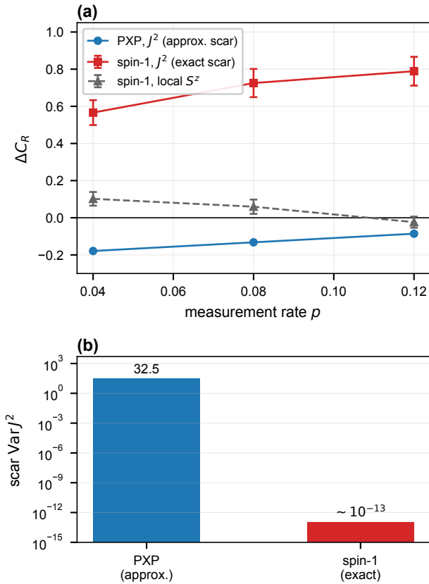
FIG. 6. Exact- \text{su}(2) scars evade the Casimir-variance obstruction. Second model (spin-1 Schechter-Iadecola, L = 6 , 20-pair thermal ensemble). (a) Scar-thermal coherent information \Delta C_R versus p (error bars are the ensemble SEM). Under J^2 monitoring PXP scars lose (blue) while exact spin-1 scars win perfectly (red); under generic local S^z the exact-scar and thermal codes are comparable at this size ( |\Delta C_R| \leq 0.1 , grey; at L = 8 the low-rate difference is larger, +0.20 at p = 0.04 , see text). (b) Scar Casimir variance, \simeq 32 (PXP, canonical rungs; 3.4–47.6 across the tower, always above energy-matched thermal neighbors) versus \sim 10^{-13} (exact) on a log scale—the control parameter of the rescue.
