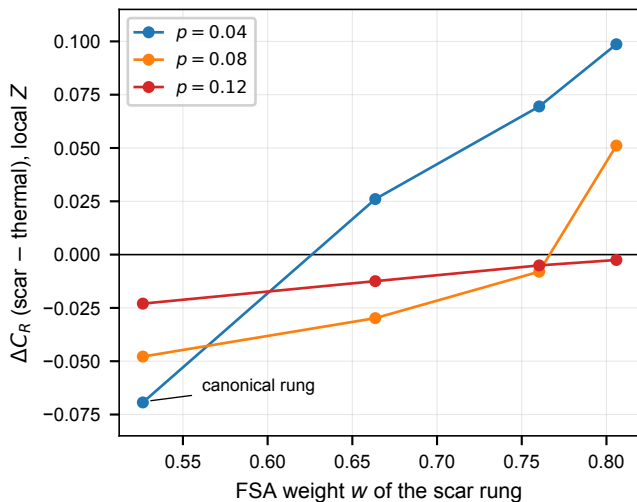
FIG. 5. Hybridization, not athermality, controls protection. Scar-minus-thermal coherent information at each energy-matchable rung of the PXP tower versus the rung’s FSA weight w (cleaned pools, L = 14 ; w increases from the canonical rung E \simeq 2.74 outward to E \simeq 6.57 ). (a) Local- Z monitoring: the deficit rises monotonically with purity and crosses to a scar advantage near w \simeq 0.65 at low rates. (b) Multiplet-binned Casimir: the same purity ordering, with bin geometry superimposed (Sec. III E).
