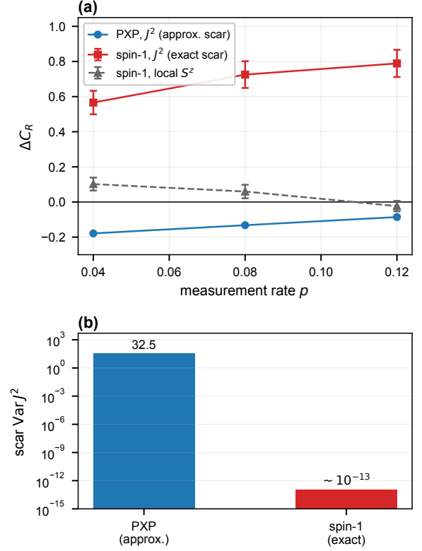
Figure 5: Exact- \text{su}(2) scars evade the Casimir-variance obstruction. Second model (spin-1 Schecter-ladecola, L = 6 , 20-pair thermal ensemble). (a) Scar-thermal coherent information \Delta\mathcal{C}_R versus p (error bars are the ensemble SEM). Under J^2 monitoring PXP scars lose (blue) while exact spin-1 scars win perfectly (red); under generic local S^z the exact-scar and thermal codes are comparable ( |\Delta\mathcal{C}_R| \lesssim 0.1 , grey). (b) Scar Casimir variance, \simeq 32 (PXP) versus \sim 10^{-13} (exact) on a log scale—the control parameter of the rescue.
