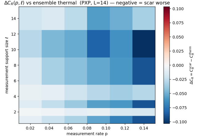
FIG. S2. \Delta\mathcal{C}_R(p, \ell) against the ensemble thermal baseline (PXP, L = 14 ). Blue is \Delta\mathcal{C}_R < 0 (scar worse) everywhere.
