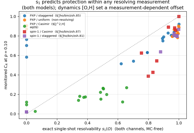
FIG. S4. Monitored \mathcal{C}_R ( p = 0.10 ) versus the exact single-shot resolvability s_1(O) for 65 code-measurement pairs across both models. Within each resolving measurement the relation is tight; the non-resolving (uniform) and non-commuting (PXP Casimir) families bound the predictor’s scope.
