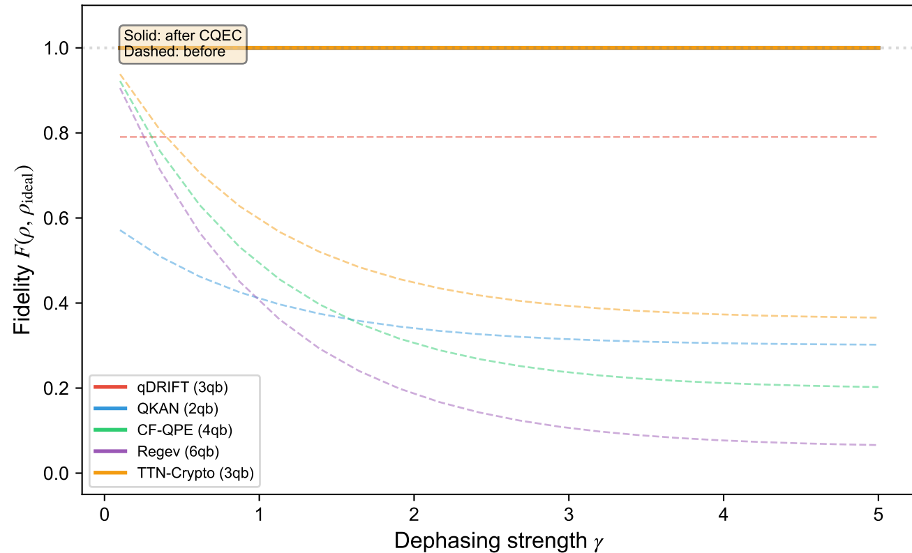
(a) Dephasing channel
