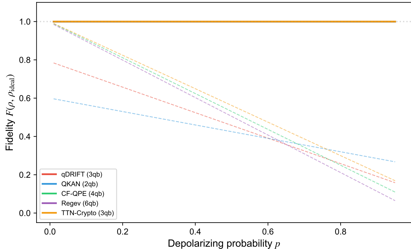
(b) Depolarizing channel
