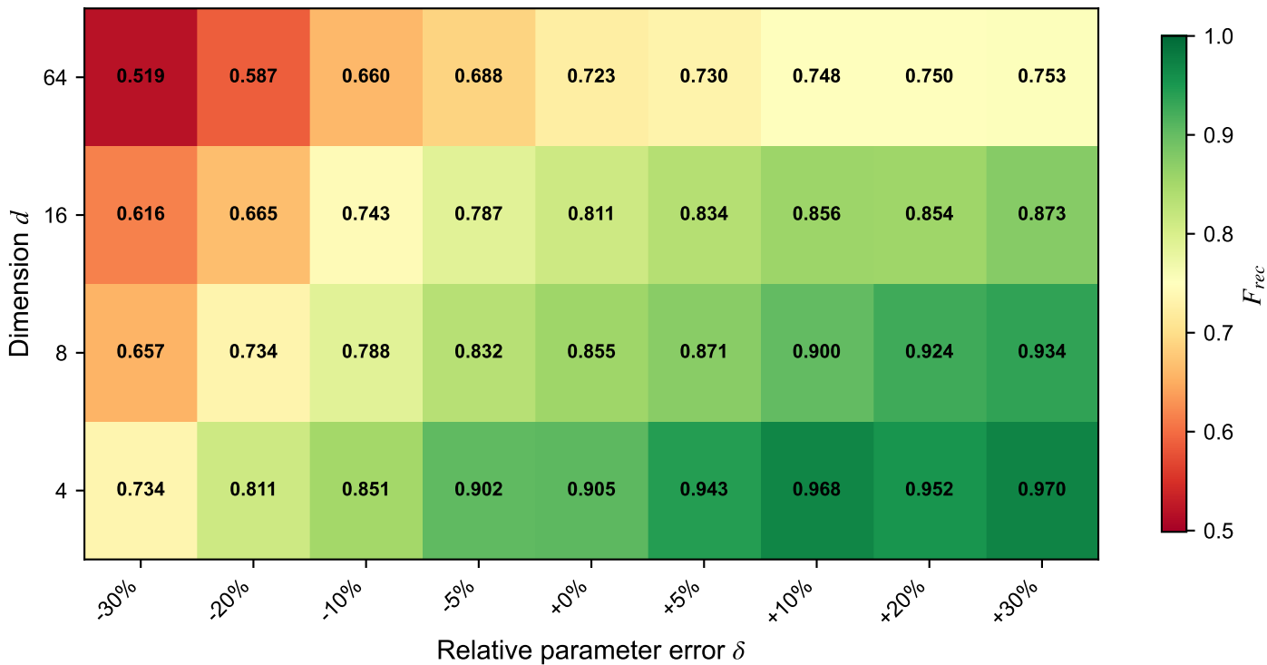
Channel-Inversion Sensitivity: F_{rec} vs Parameter Error (all params shifted simultaneously, 10 Haar-random states)
