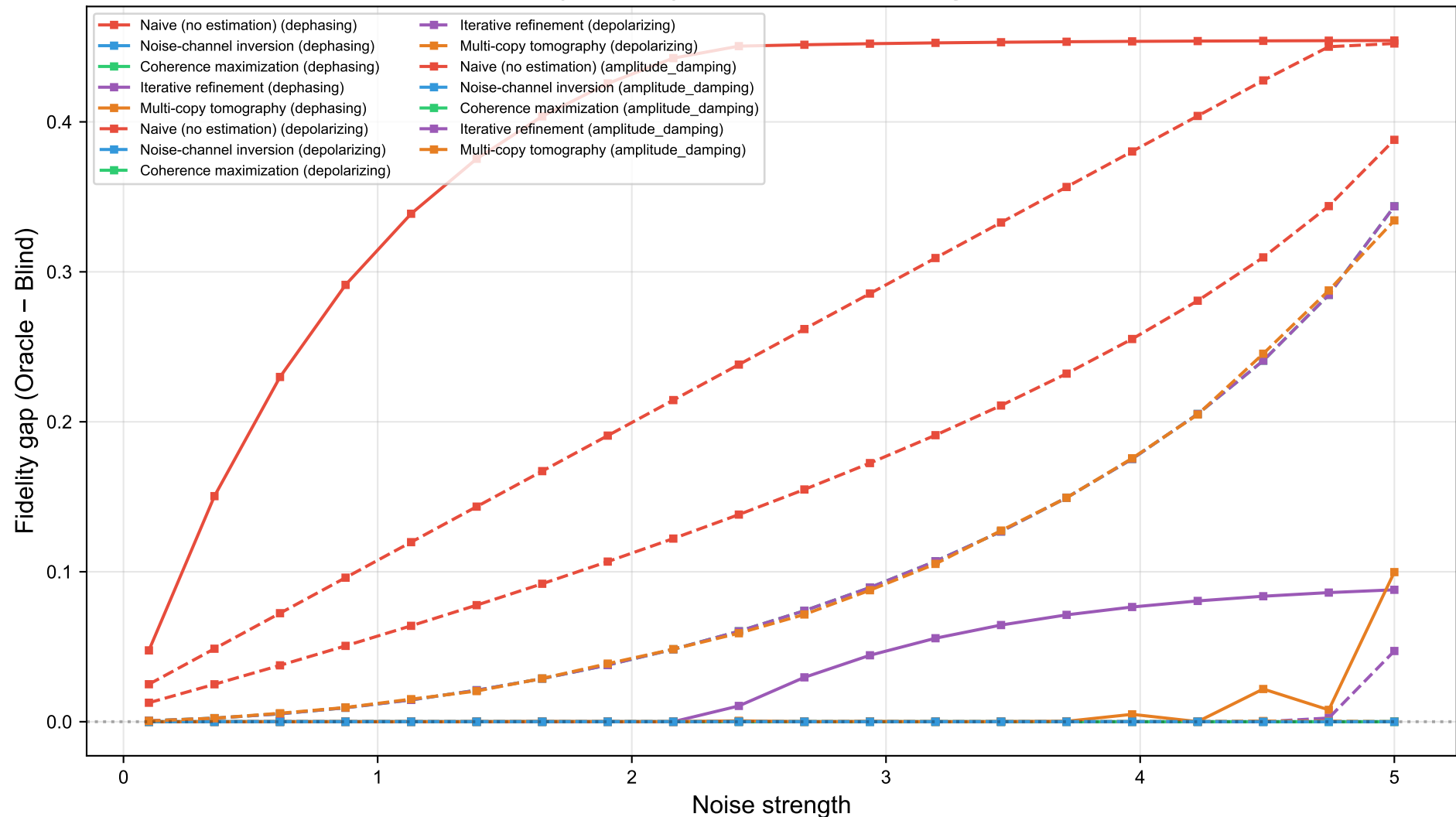
Fidelity Penalty from Unknown Target State
