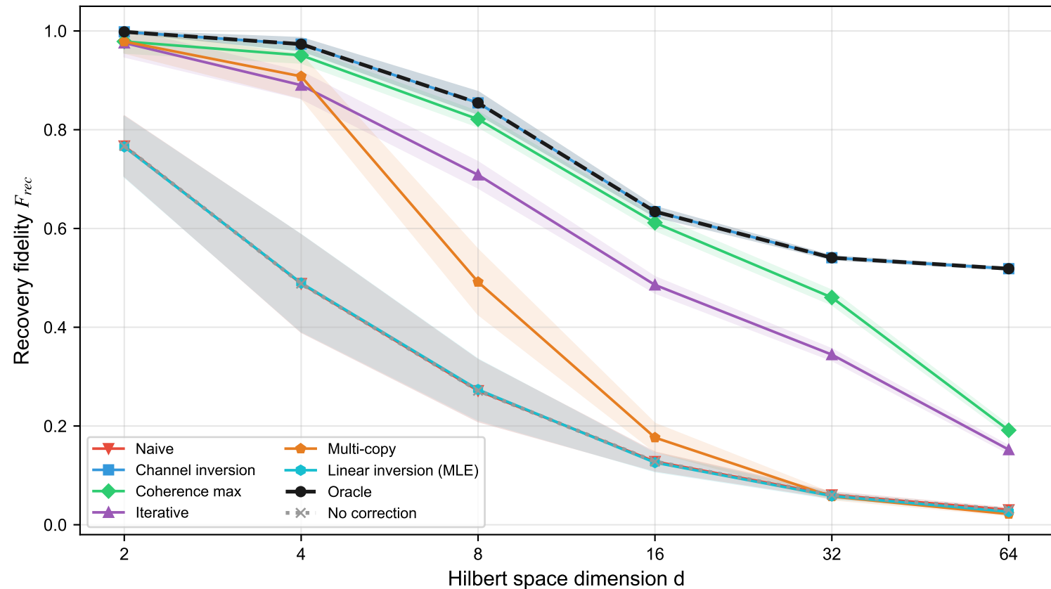
Blind CQEC: Dimension Sweep with Haar-Random States (20 states/dim, combined noise: dephasing+depolarizing+amp. damping)
