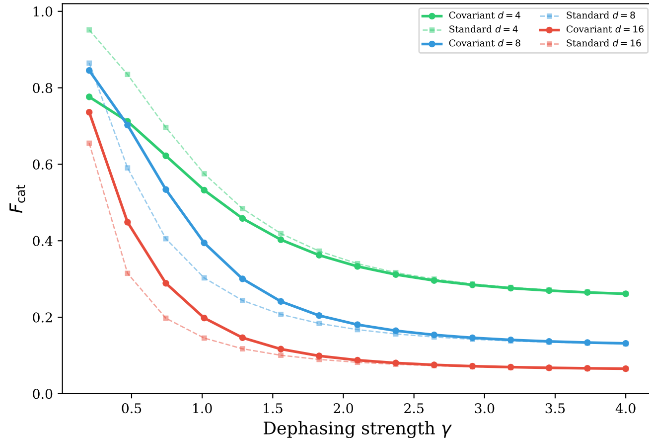
(a) F_{\text{cat}} vs. \gamma ( n = 8 copies)
