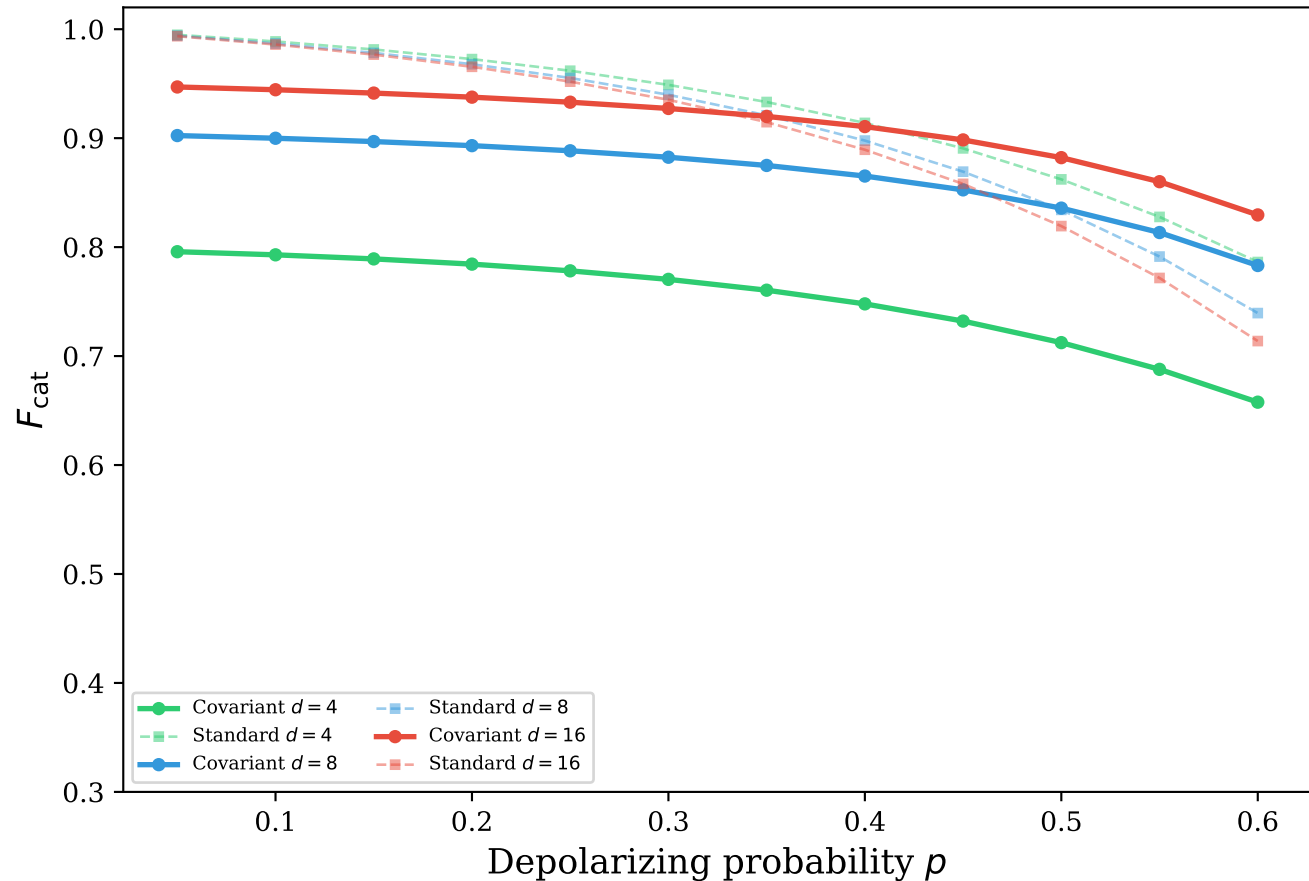
(b) F_{\text{cat}} vs. p ( n = 8 copies)
