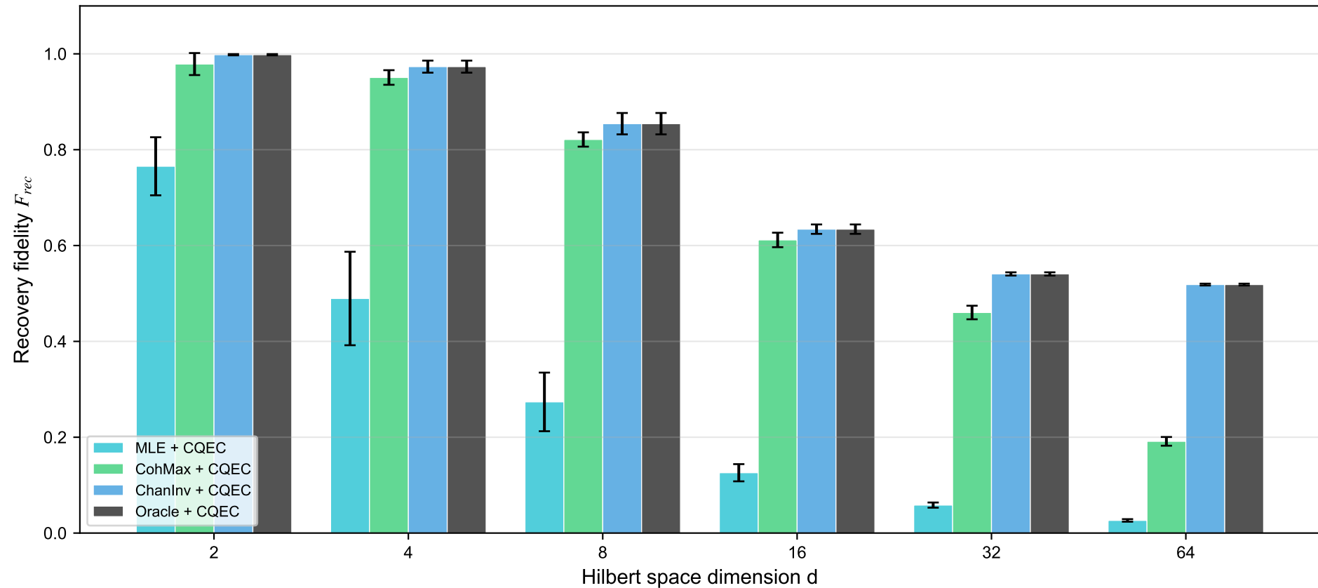
MLE vs Coherence-Max vs Channel-Inversion + CQEC (mean \pm std over 20 Haar-random states)
