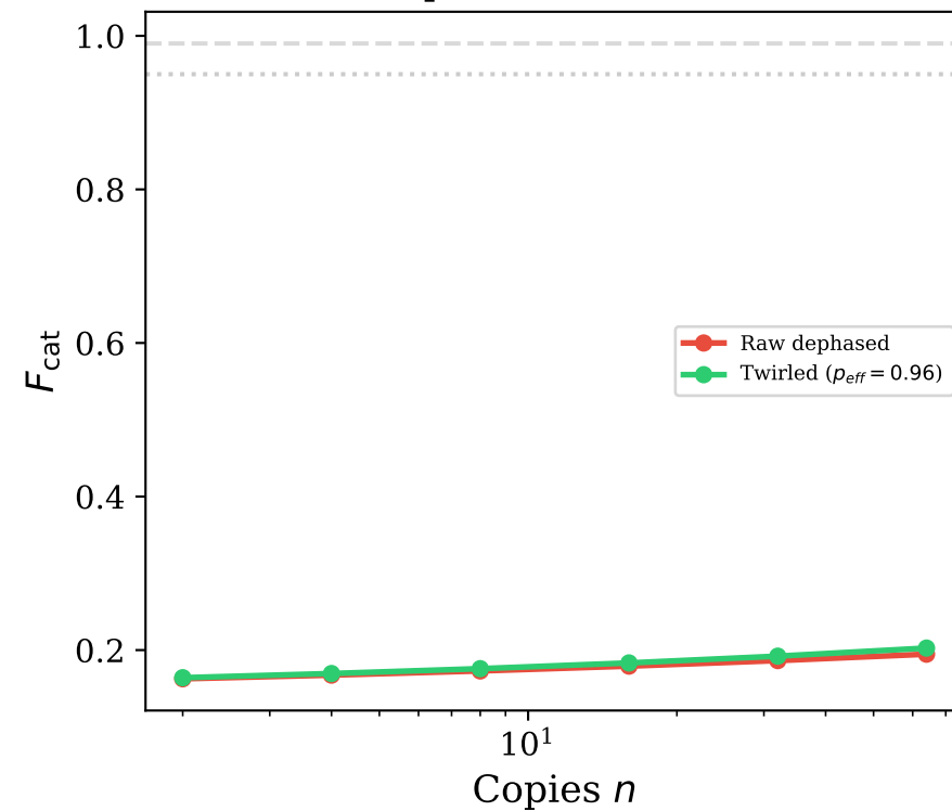
qDRIFT ( d = 8 )
