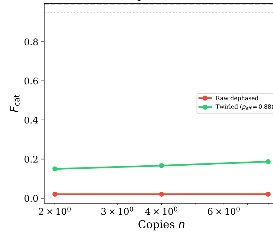
Regev ( d = 64 )
