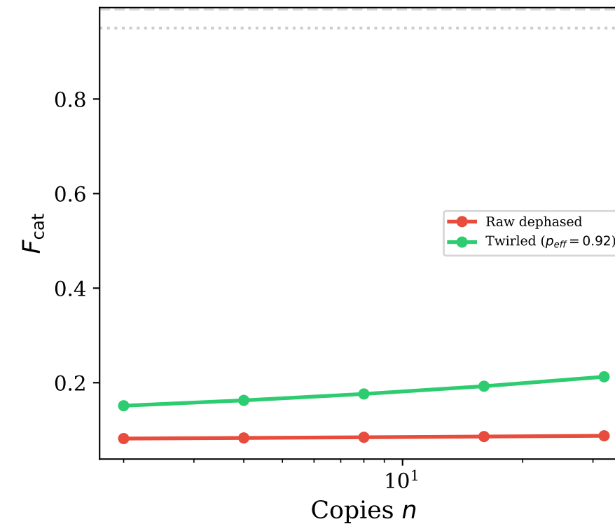
CF-QPE ( d = 16 )
