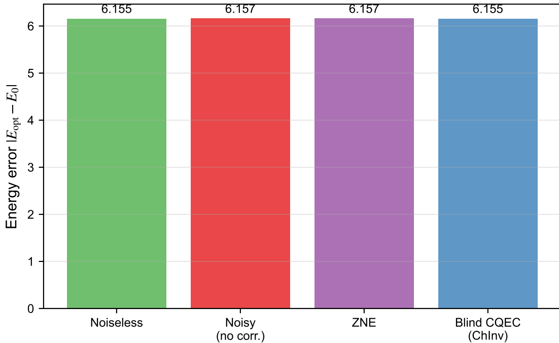
LiH-like Hamiltonian ( d=16 ) VQE
