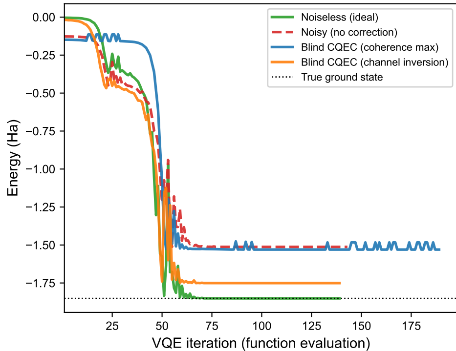
(a) VQE convergence
