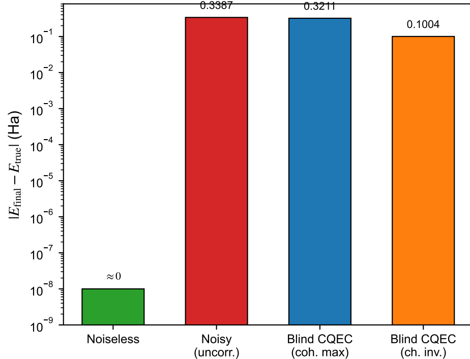
(b) Final energy error
