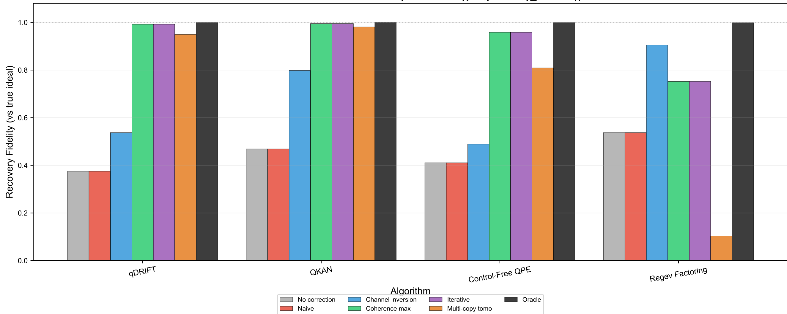
Blind CQEC: Combined Noise ( \gamma=1, p=0.15, \gamma_{AD}=0.1 )
