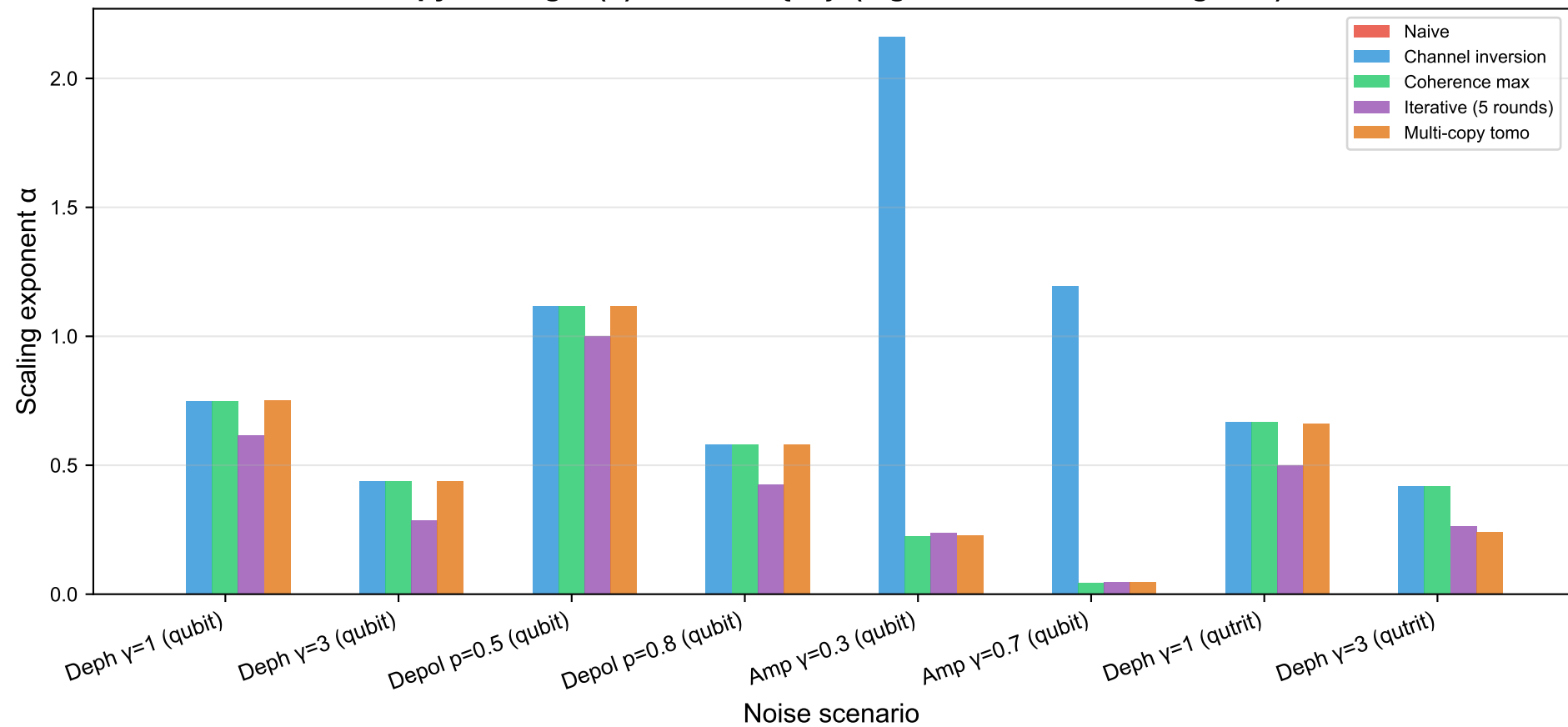
Copy Scaling: F(n) \sim 1 - A \cdot n^{-\alpha} (higher \alpha = faster convergence)
