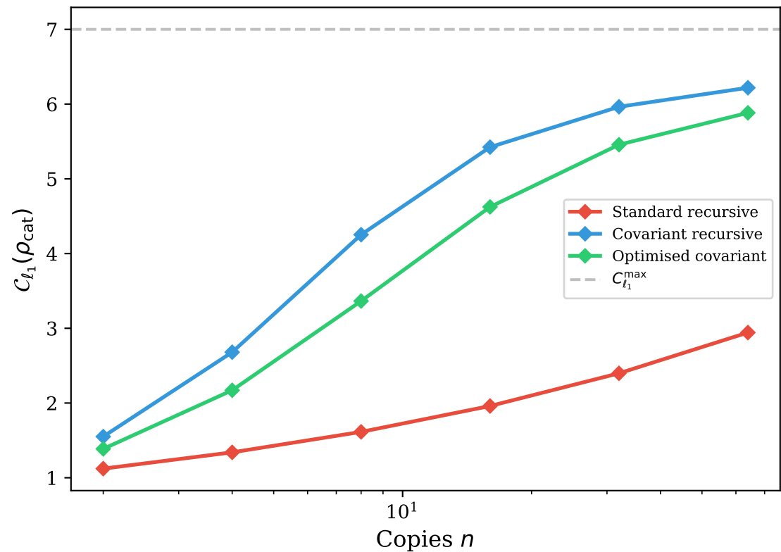
d = 8 , coherence under dephasing
