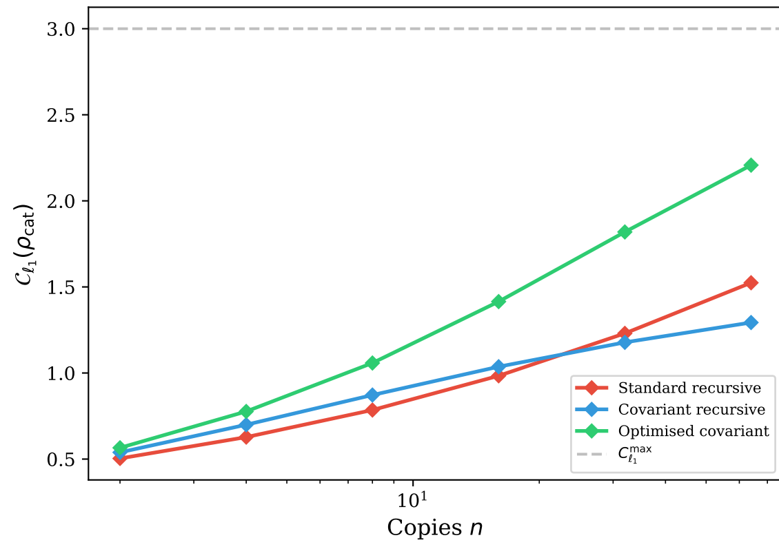
d = 4 , coherence under dephasing
