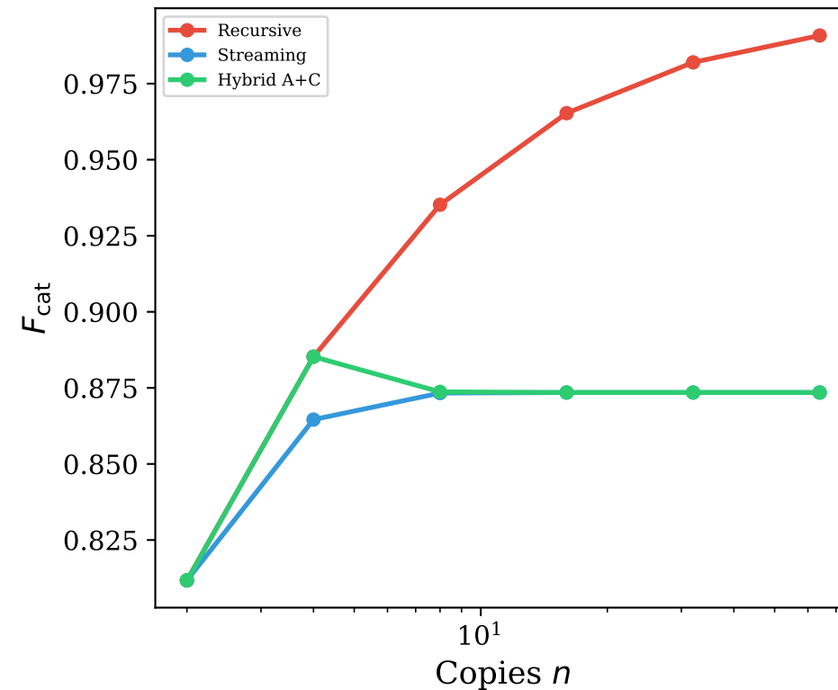
CF-QPE ( d = 16 )
