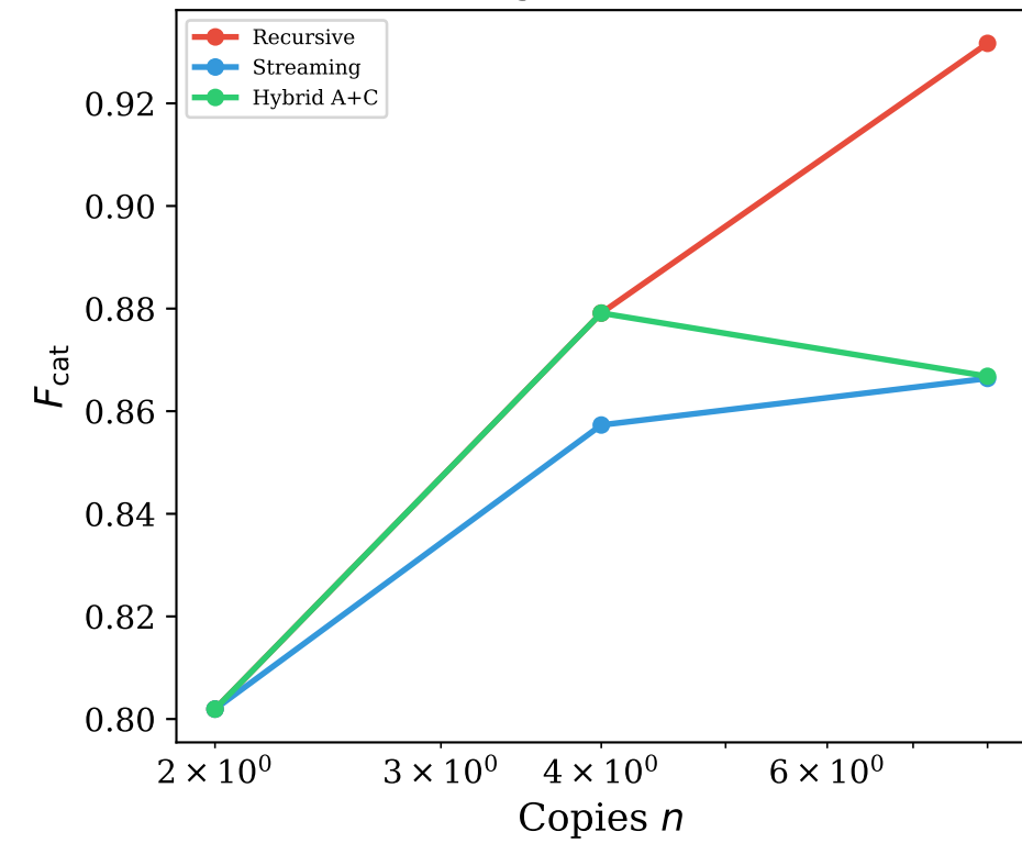
Regev ( d = 64 )
