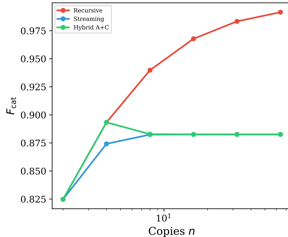
qDRIFT ( d = 8 )
