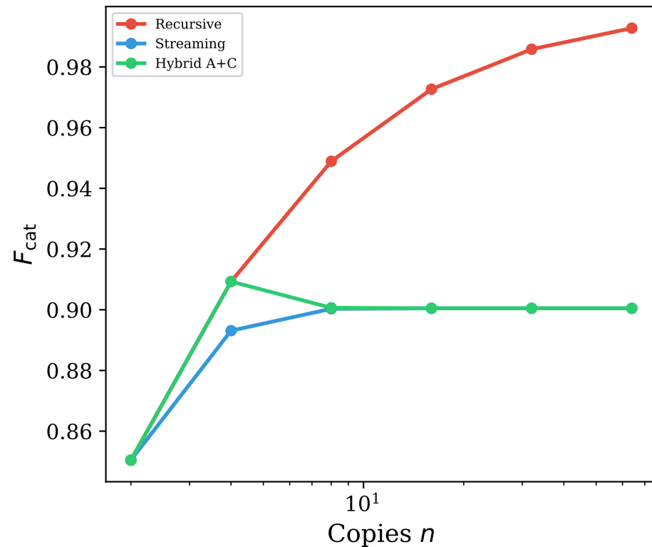
QKAN ( d = 4 )
