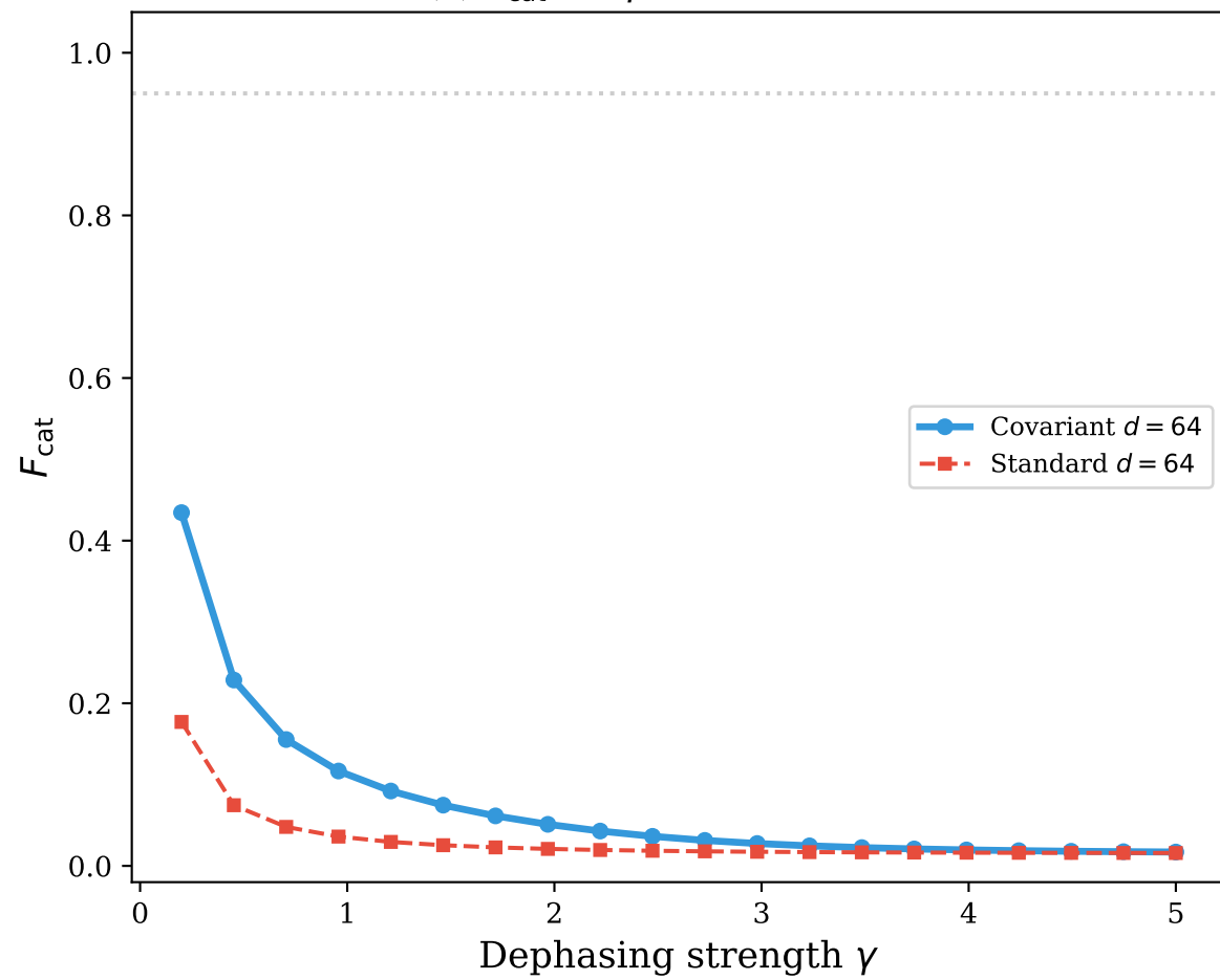
(c) F_{\text{cat}} vs. \gamma at d = 64, n = 8
