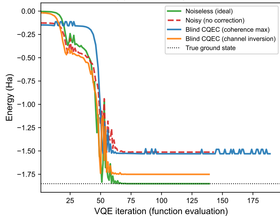
(a) VQE convergence
