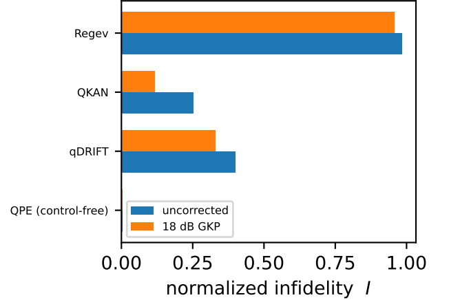
FIG. 2. Unit-independent normalized infidelity I (uncorrected vs 18 dB).
