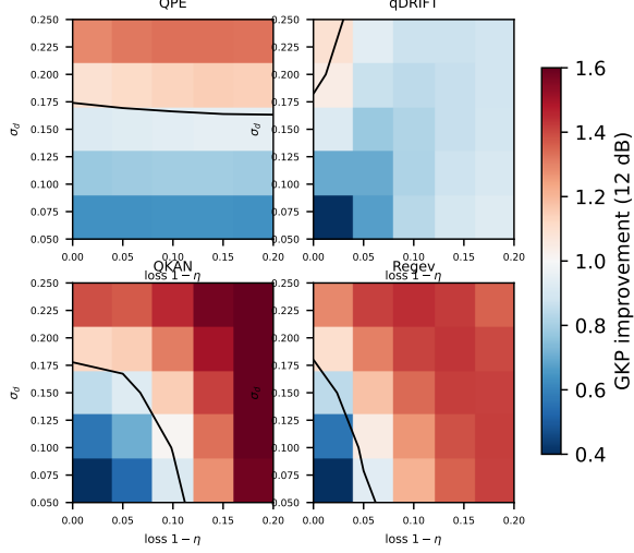
FIG. 3. GKP improvement factor (12 dB) over the (\sigma_d, \text{loss}) plane; black contour marks the floor crossing (improvement = 1). Blue: GKP helps; red: counterproductive (below the squeezing floor).
