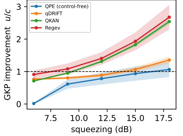
FIG. 1. GKP improvement factor vs squeezing (dB) at \sigma_d = 0.10 , loss 0.15; shaded band = 95% CI over 10 seeds. The floor crossing (improvement = 1) confirms Prop. 1.
