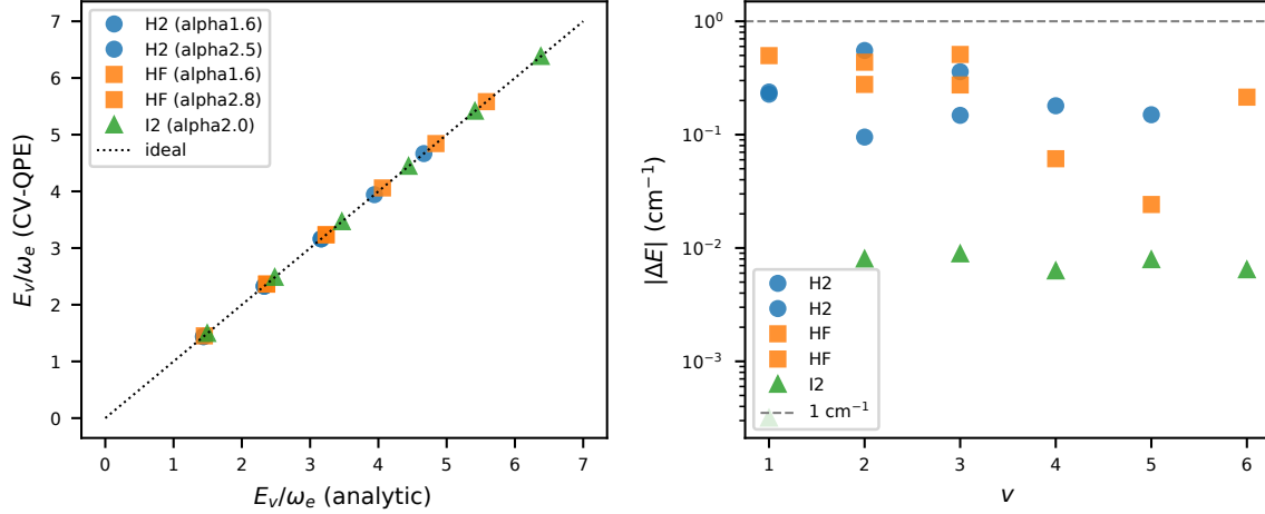
Figure 4. CV control-free QPE applied to three diatomic Morse vibrational spectra (H 2 , HF, I 2 ). Left : recovered vs analytic E_v/\omega_e for the runs of Table 4; the dotted line is the ideal. Right : absolute energy error vs v in cm -1 , log scale; every point sits below the 1 cm -1 spectroscopic threshold (grey dashed), with I 2 reaching \sim 10^{-2} cm -1 .
