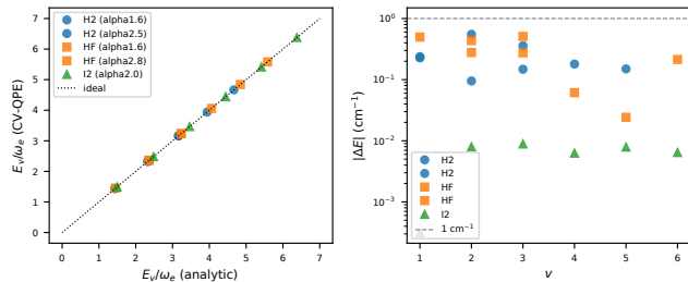
FIG. 4. CV control-free QPE applied to three diatomic Morse vibrational spectra (H 2 , HF, I 2 ). Left : recovered vs analytic E_v/\omega_e for the runs of Table IV; the dotted line is the ideal. Right : absolute energy error vs v in cm -1 , log scale; every point sits below the 1 cm -1 spectroscopic threshold (grey dashed), with I 2 reaching \sim 10^{-2} cm -1 .
