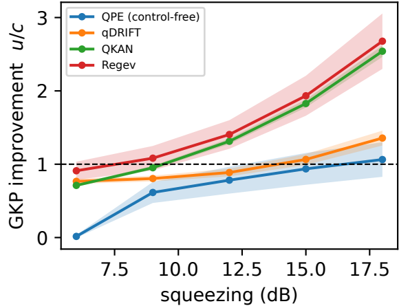
FIG. 1. GKP improvement factor vs squeezing (dB) at \sigma_d = 0.10 , loss 0.15; shaded band = 95% CI over 10 seeds. The floor crossing (improvement = 1) confirms Prop. 1.
