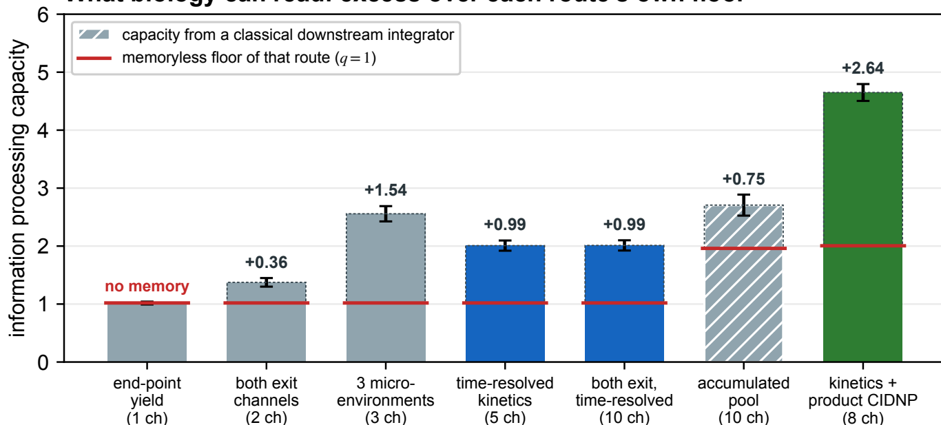
Fig. 2 Readout is not the bottleneck. Capacity recovered by chemically accessible observables at the cryptochrome operating point ( B = 50 \mu\text{T} , J = 0 , \tau = 1 \mu\text{s} ), with spin-selective recombination switched on so that the observable is the product actually formed. All seven routes defined by the model are shown. Red bars mark each route's own memoryless floor, measured by wiping the nuclear register every cycle ( q = 1 ); these are not common to the routes (1.02 for the yield routes, 2.01 for the eight-channel CIDNP route, 1.96 for the accumulated pool), so it is the dashed excess above each floor—printed above each bar—that measures memory, not the bar height. Ordinary reaction kinetics clear their floor by 0.99, and the nuclear polarisation carried away by the product—chemically induced dynamic nuclear polarisation, CIDNP 18 —clears its own by 2.64, the largest of any route. The end-point yield sits exactly on its floor: it reports the present input and remembers nothing. The accumulated pool is hatched because a leaky downstream integrator is itself a classical delay line, so its excess is not evidence of nuclear-spin memory. No spectroscopy is involved.
