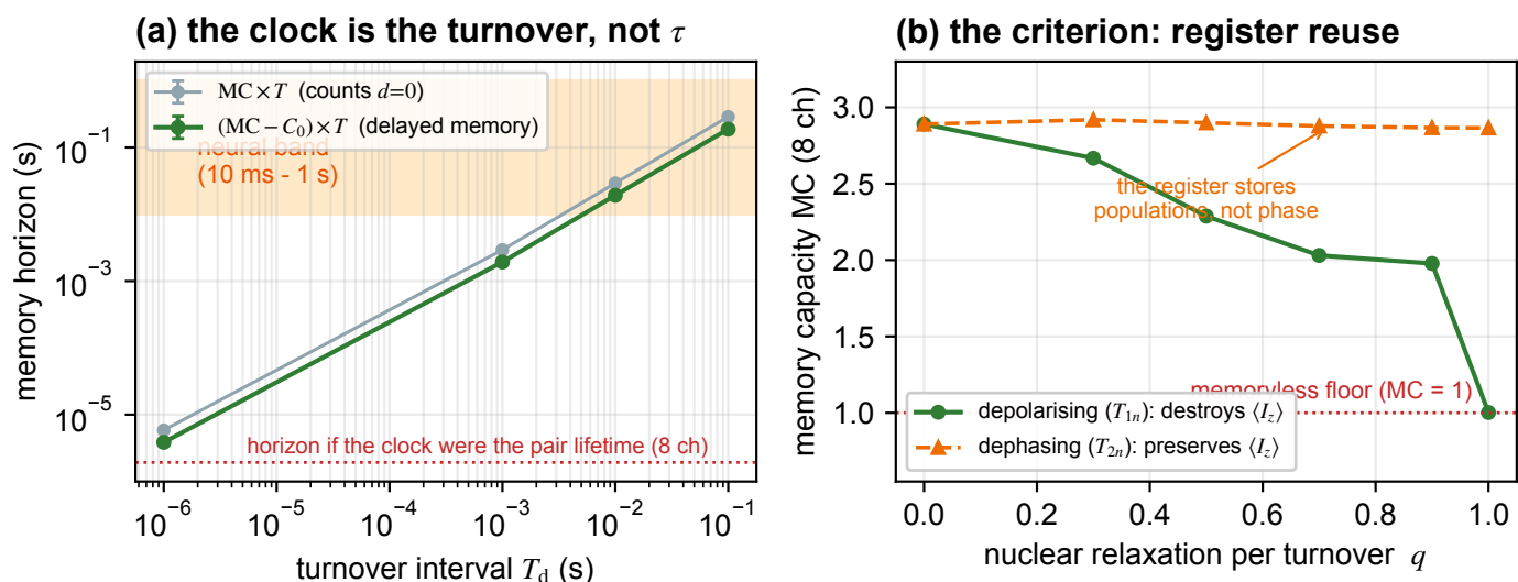
Fig. 3 (a) The memory horizon against the turnover interval, from twelve input realisations (error bars are the between-seed standard deviation). Because the nuclear register survives recombination, inserting a physiological pause costs only 1.6% of the memory capacity across five decades, so the horizon simply tracks the clock and enters the neural band (shaded, 10 ms–1 s, the range of cortical rhythms 8 ). Both definitions are shown: the raw MC \times T_{\text{turnover}} (grey) counts the zero-delay term, which carries no memory, while the delayed-memory horizon (MC - C_0) \times T_{\text{turnover}} (green) is the quantity quoted in the text—on the latter the 1 ms turnover falls below the band. The dotted line is where the horizon would sit if the clock were the radical-pair lifetime, for the same eight-channel readout. (b) The criterion, and which relaxation process enforces it. Depolarising the register between turnovers with probability q (green) drives the capacity to the memoryless floor: at q = 1 —a fresh molecule each cycle— MC = 1.00 and there is no memory. Pure nuclear dephasing at the same q (orange) leaves MC = 2.87 , essentially untouched: the register stores populations, not phase, so the constant that bounds the horizon is T_{1n} . Note that this does not lengthen the horizon at the operating point, where extreme narrowing brings T_{1n} and T_{2n} together (ESI, Sec. S12).
