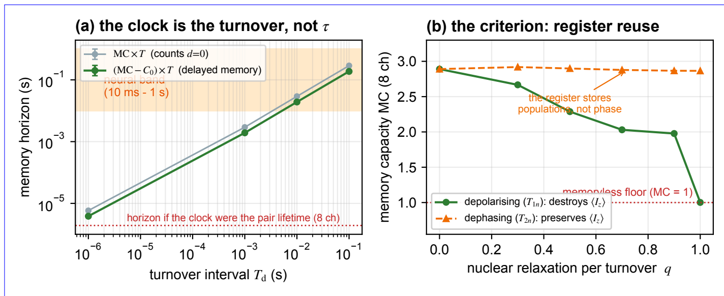
Fig. 3 (a) The memory horizon against the turnover interval, from twelve input realisations (error bars are the between-seed standard deviation). Because the nuclear register survives recombination, inserting a physiological pause costs only 1.6% of the memory capacity across five decades, so the horizon simply tracks the clock and enters the neural band (shaded, 10 ms–1 s, the range of cortical rhythms 8 ). Both definitions are shown: the raw MC \times T_{\text{turnover}} (grey) counts the zero-delay term, which carries no memory, while the delayed-memory horizon (MC - C_0) \times T_{\text{turnover}} (green) is the quantity quoted in the text—on the latter the 1 ms turnover falls below the band. The dotted line is where the horizon would sit if the clock were the radical-pair lifetime, for the same eight-channel readout. (b) The criterion, and which relaxation process enforces it. Depolarising the register between turnovers with probability q (green) drives the capacity to the memoryless floor: at q = 1 —a fresh molecule each cycle— MC = 1.00 and there is no memory. Pure nuclear dephasing at the same q (orange) leaves MC = 2.87 , essentially untouched: the register stores populations, not phase, so the constant that bounds the horizon is T_{1n} . Note that this does not lengthen the horizon at the operating point, where extreme narrowing brings T_{1n} and T_{2n} together (ESI, Sec. S12).
