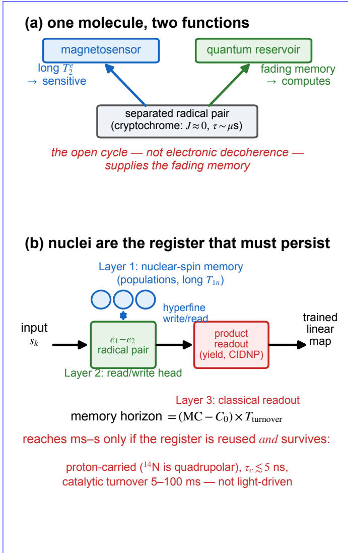
Fig. 1 The reservoir and the quantity that decides its reach. (a) A cryptochrome-type separated radical pair ( J \approx 0 , lifetime \tau \sim \mu\text{s} ) is the same molecule in two roles: long electronic coherence makes it a weak-field magnetosensor, while the dissipation of an open cycle supplies the fading memory a reservoir needs. (b) The nuclei are the register: they are not consumed by recombination and therefore persist from one turnover to the next, whereas the electron pair is created afresh each cycle. The memory horizon is consequently set by T_{\text{turnover}} and not by \tau , and is quoted throughout as (MC - C_0) \times T_{\text{turnover}} , the zero-delay term C_0 \simeq 1 carrying no memory. It reaches the neural band only if the register is genuinely reused and survives the pause, which requires it to be carried by protons rather than the quadrupolar flavin ^{14}\text{N} and to reorient with \tau_c \lesssim 6 ns (ESI, Secs. S9 and S12).
