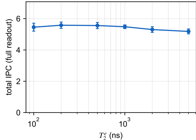
(a) real cryptochrome @ 50 \mu\text{T}
