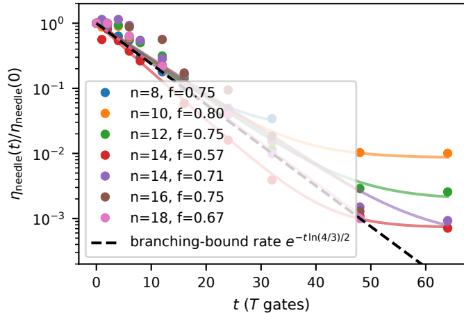
(a) collapse vs branching-bound rate, n = 8-18
