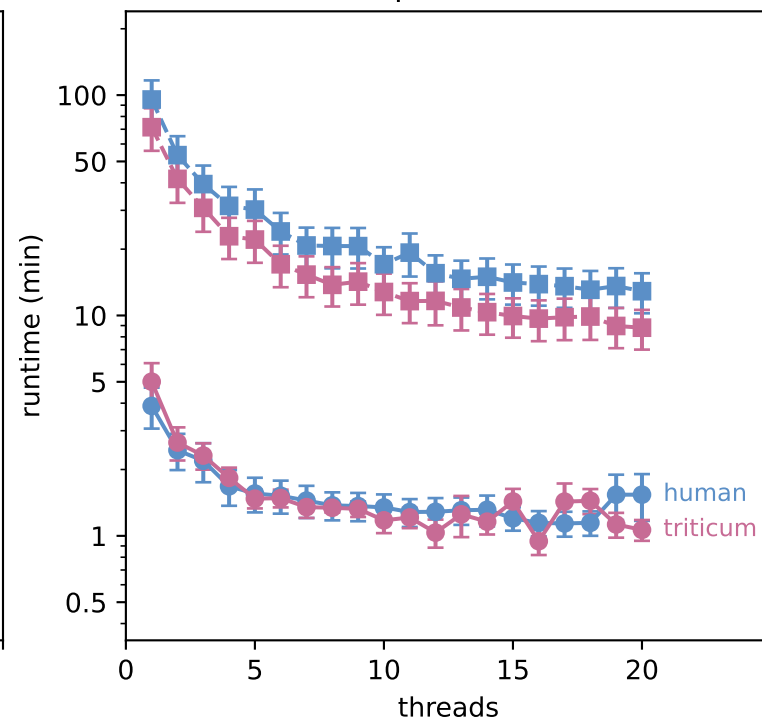
computematrix
