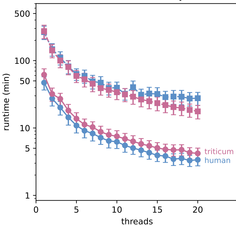
multibamssummary
