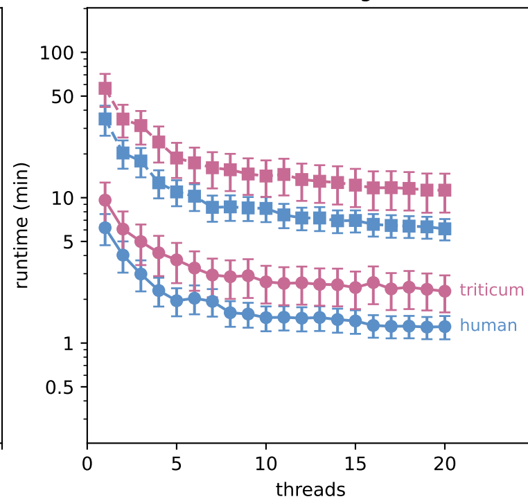
computematrix
