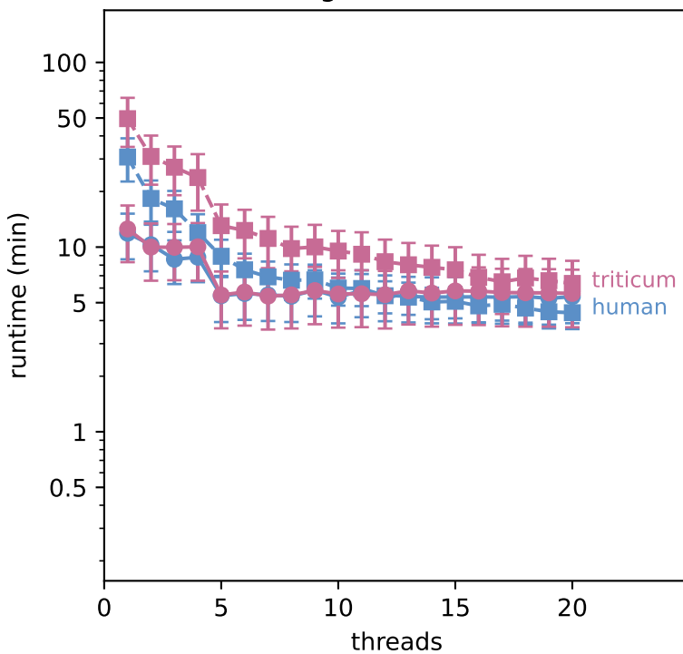
multibamssummary
