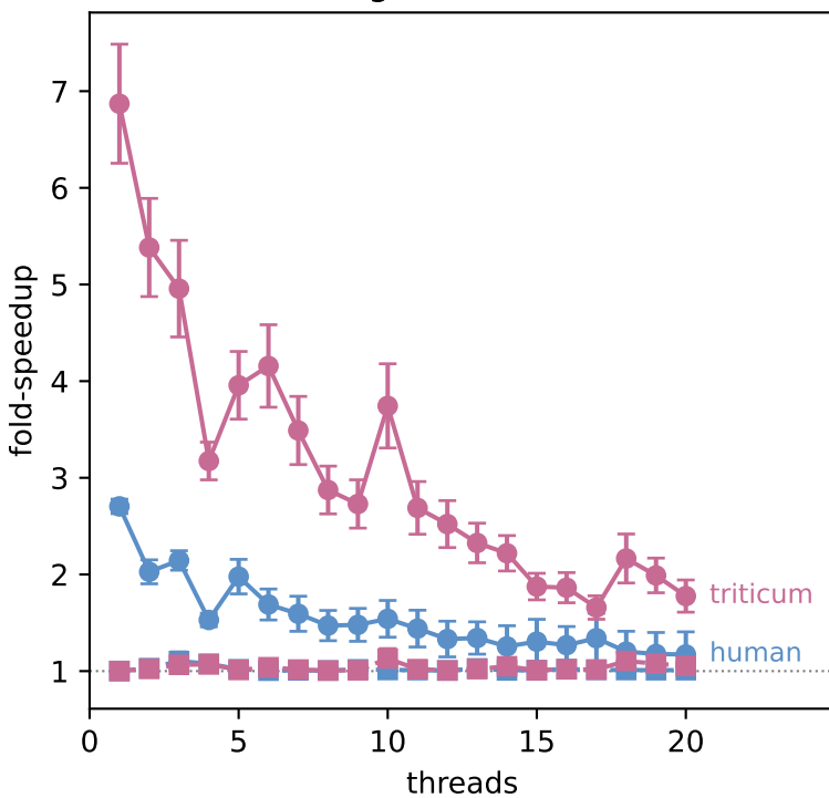
multibamsummary
