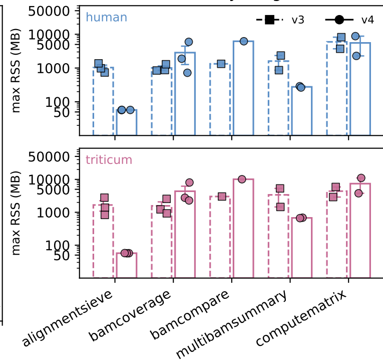
memory usage
