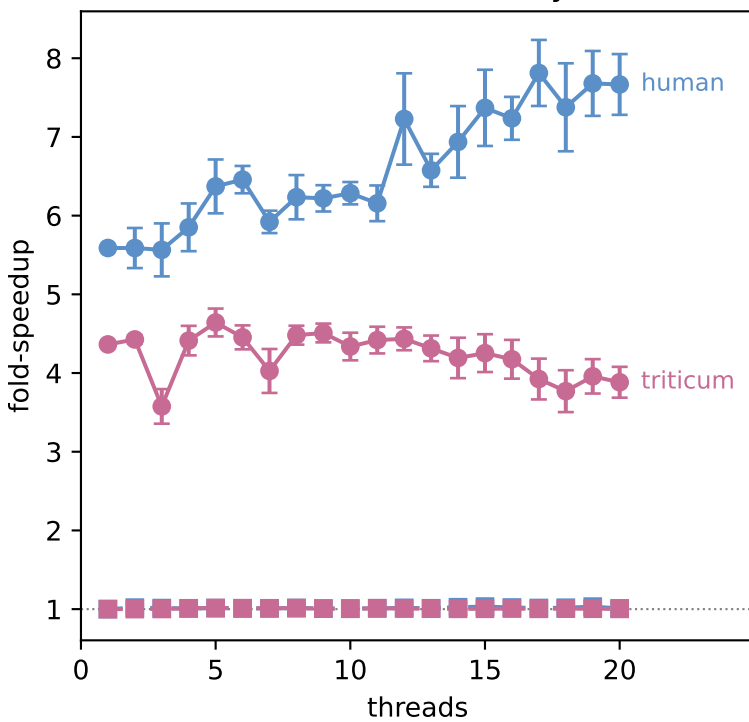
multibamsummary
