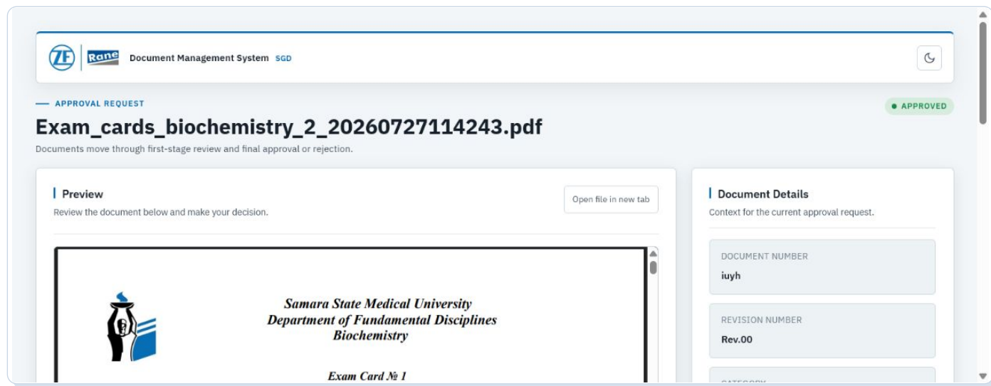
Figure 7 - Approval review workspace with preview and document details
