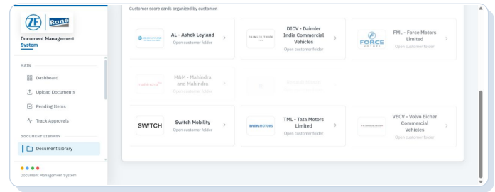
Figure 13 - Customer Records
