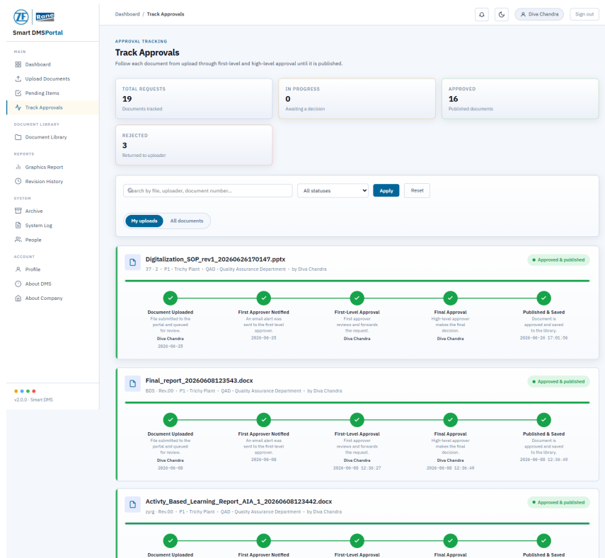
Figure 7: Approval tracking with status stepper and document history.
