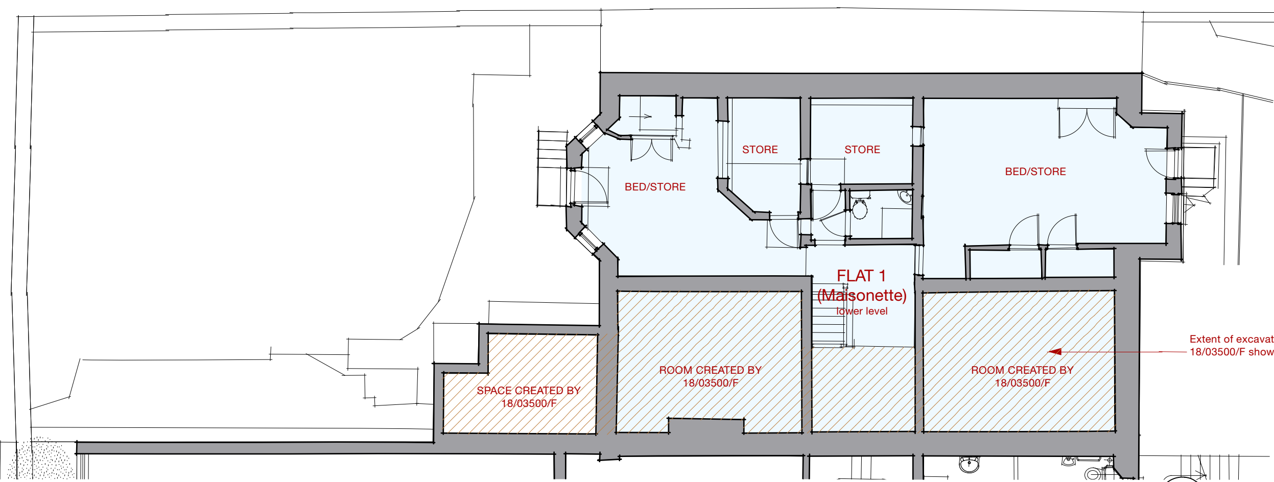
1 Lower Ground Floor Plan Scale: 1:100
