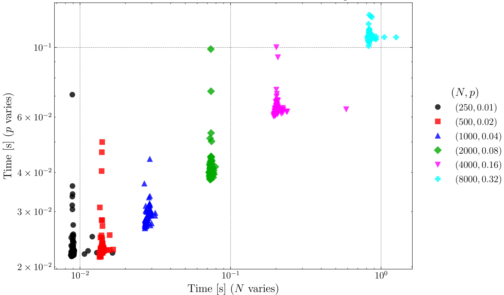
Performance Correlation Between N and p
